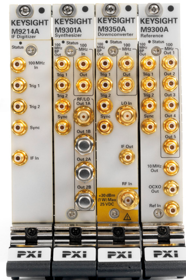
Figure 1. M9391A PXIe vector signal analyzer with four modules consisting of the M9214A digitizer, M9301A synthesizer, M9350A downconverter and M9300A frequency reference.
