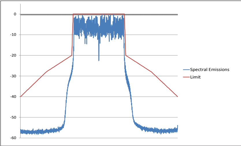
Figure 10. WLAN 802.11ac SEM at 5.8 GHz, 80 MHz bandwidth.
