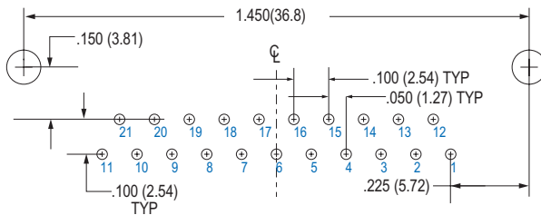
21 PIN M83513/16-C
