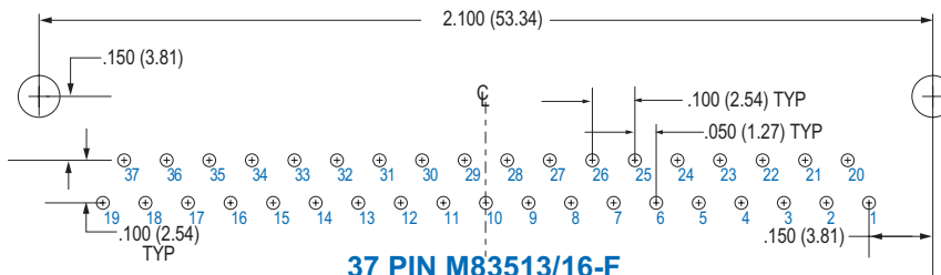
37 PIN M83513/16-F
