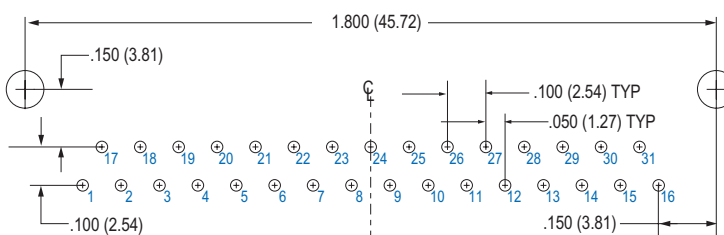
31 SOCKET M83513/19-E
