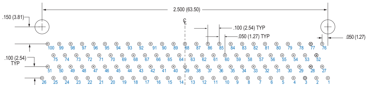
100 PIN M83513/18-H
