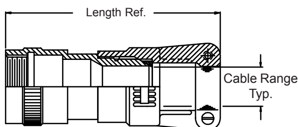
Function "D" Adapter Assembly
