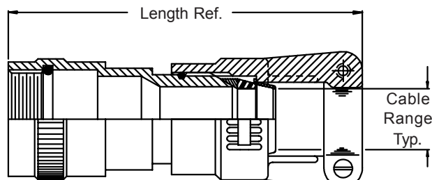
Function "B" Adapter Assembly
