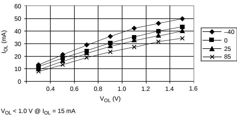
Figure 23-9. Typical Low-Side Driver Characteristics – Port PTC1–PTC0 ( V_{DD} = 4.5\text{ Vdc} )
