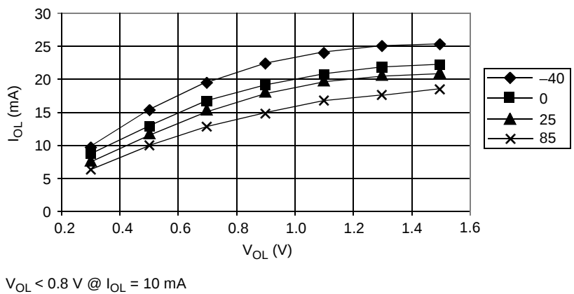
Figure 23-10. Typical Low-Side Driver Characteristics – Port PTC1–PTC0 ( V_{DD} = 2.7\text{ Vdc} )
