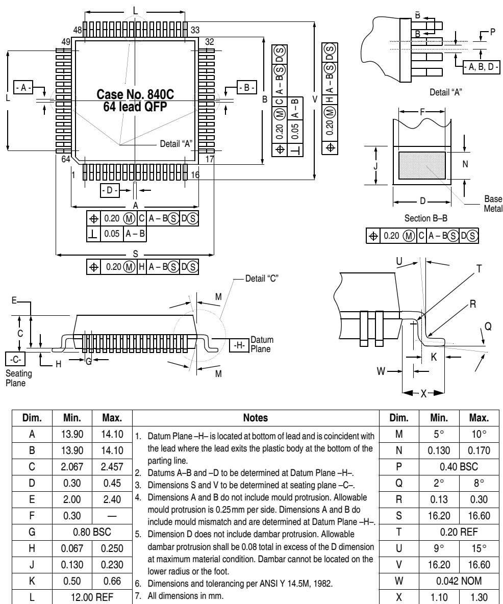
Figure 12-5 64-pin QFP mechanical dimensions
