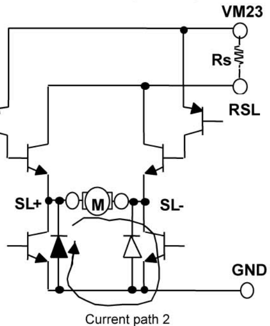
FORWARD Current path timing 2.
