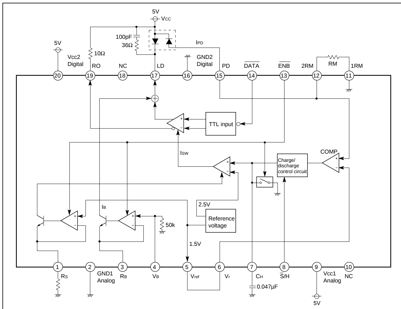
Figure 1 Example of Sample-and-Hold Type APC Circuit Application
