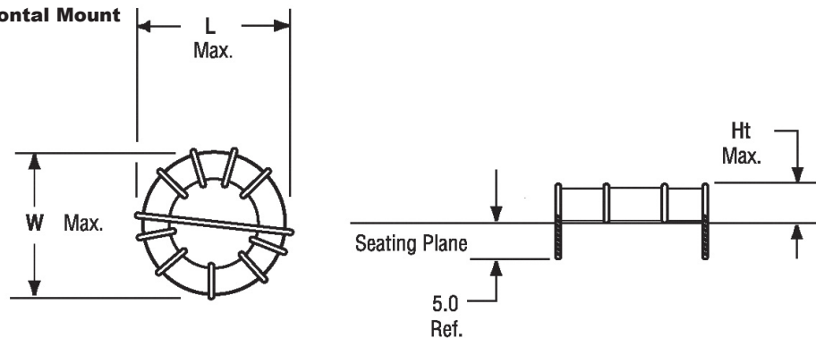
Figure 2 Horizontal Mount
