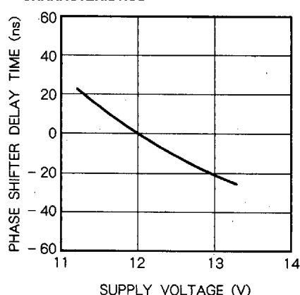
PHASE SHIFTER DELAY TIME - SUPPLY VOLTAGE CHARACTERISTICS
