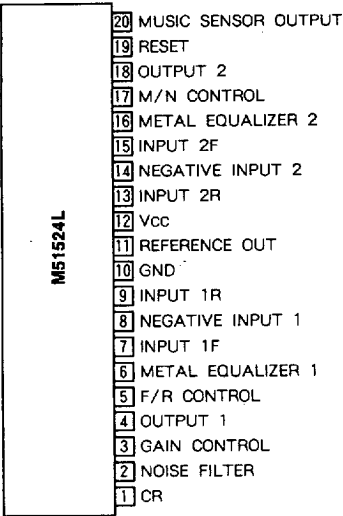
Outline 20P5A(L)
