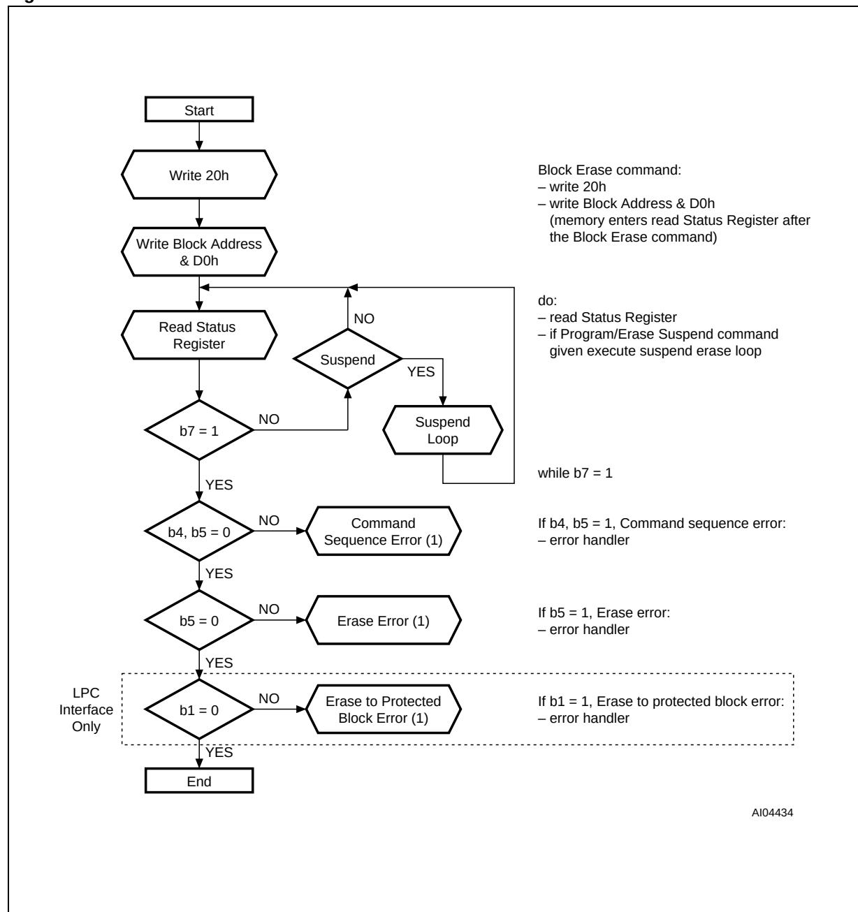
Figure 17. Block Erase Flowchart and Pseudo Code
