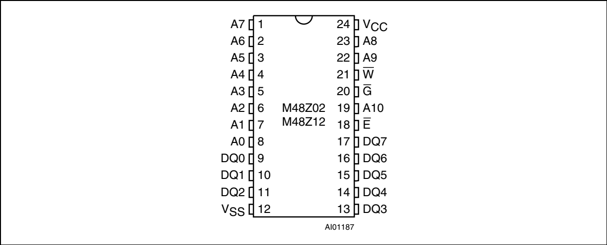
Figure 2. DIP connections
