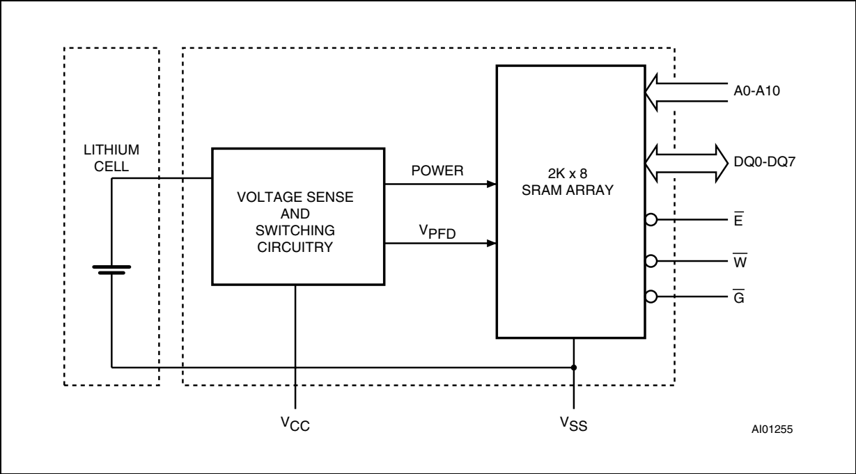
Figure 3. Block diagram
