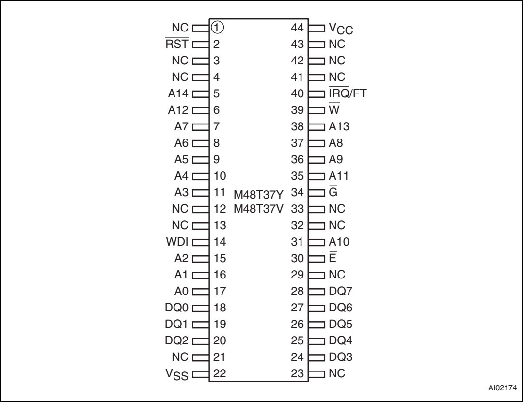
Figure 2. SOIC connections
