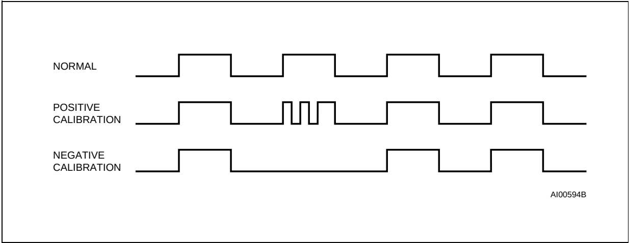
Figure 10. Clock Calibration
