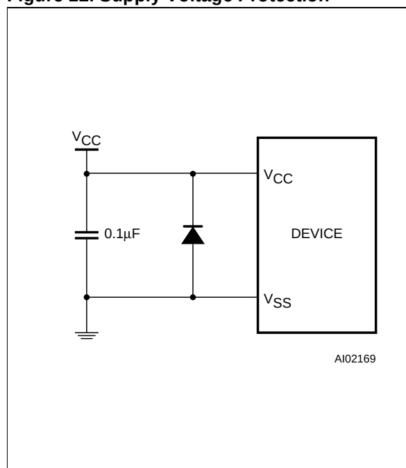
Figure 12. Supply Voltage Protection
