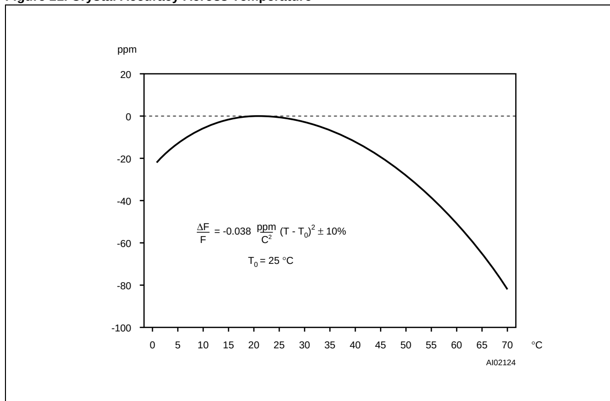
Figure 11. Crystal Accuracy Across Temperature
