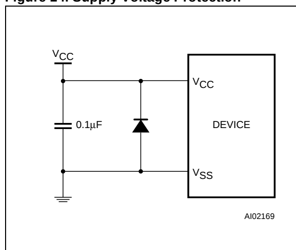
Figure 14. Supply Voltage Protection
