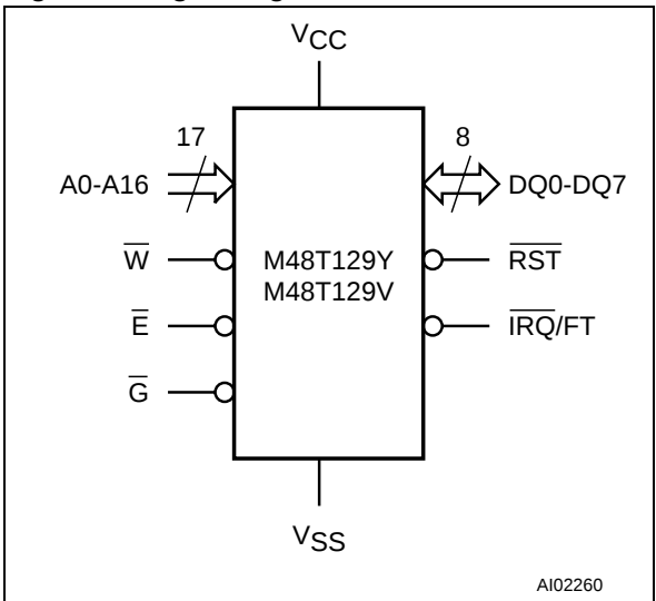
Figure 2. Logic Diagram
