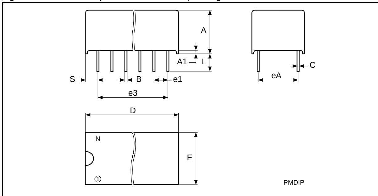
Figure 17. PMDIP32 – 32-pin Plastic DIP Module, Package Outline
