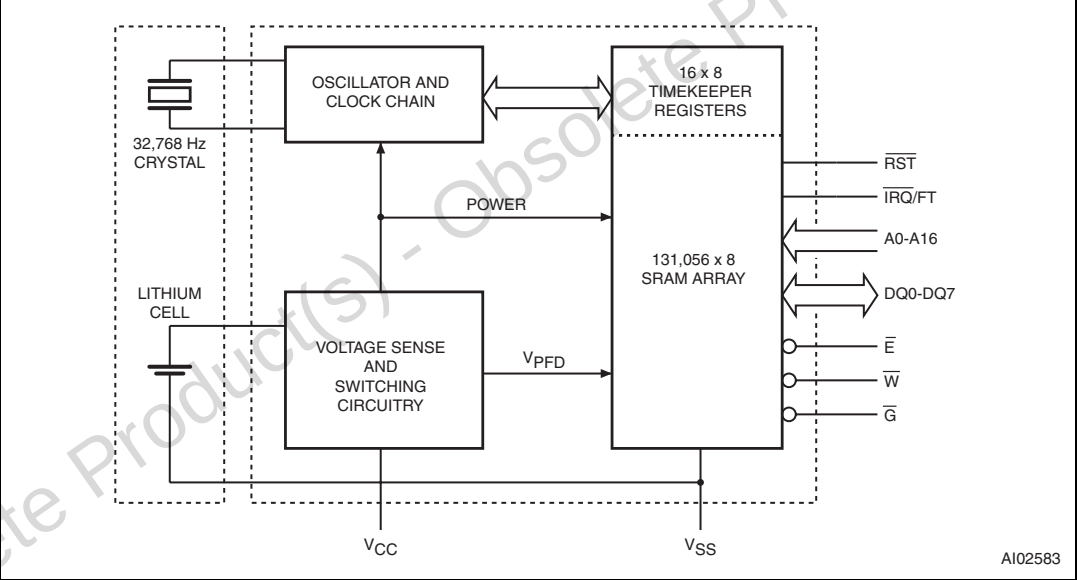
Figure 3. Block diagram
