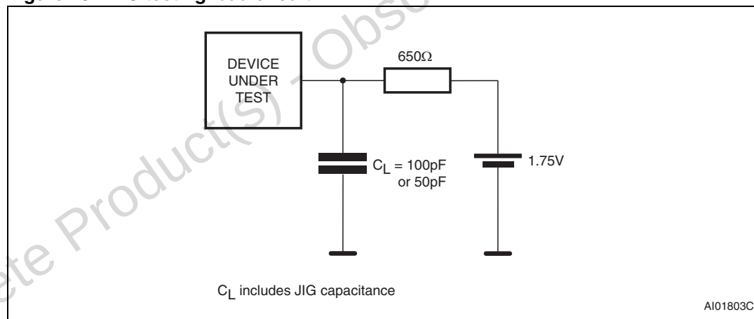
Figure 13. AC testing load circuit
