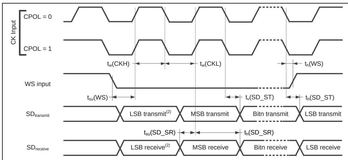
Figure 9.6-6 I²S Slave Mode Timing Diagram
