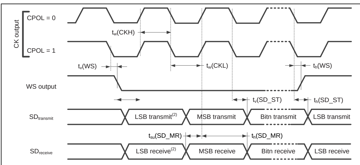
Figure 9.6-3 I 2 S Master Mode Timing Diagram
