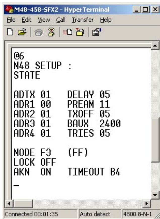
Figure 3: M48 Setup Mode screen output to STATE command when Acknowledgement Mode is enabled
