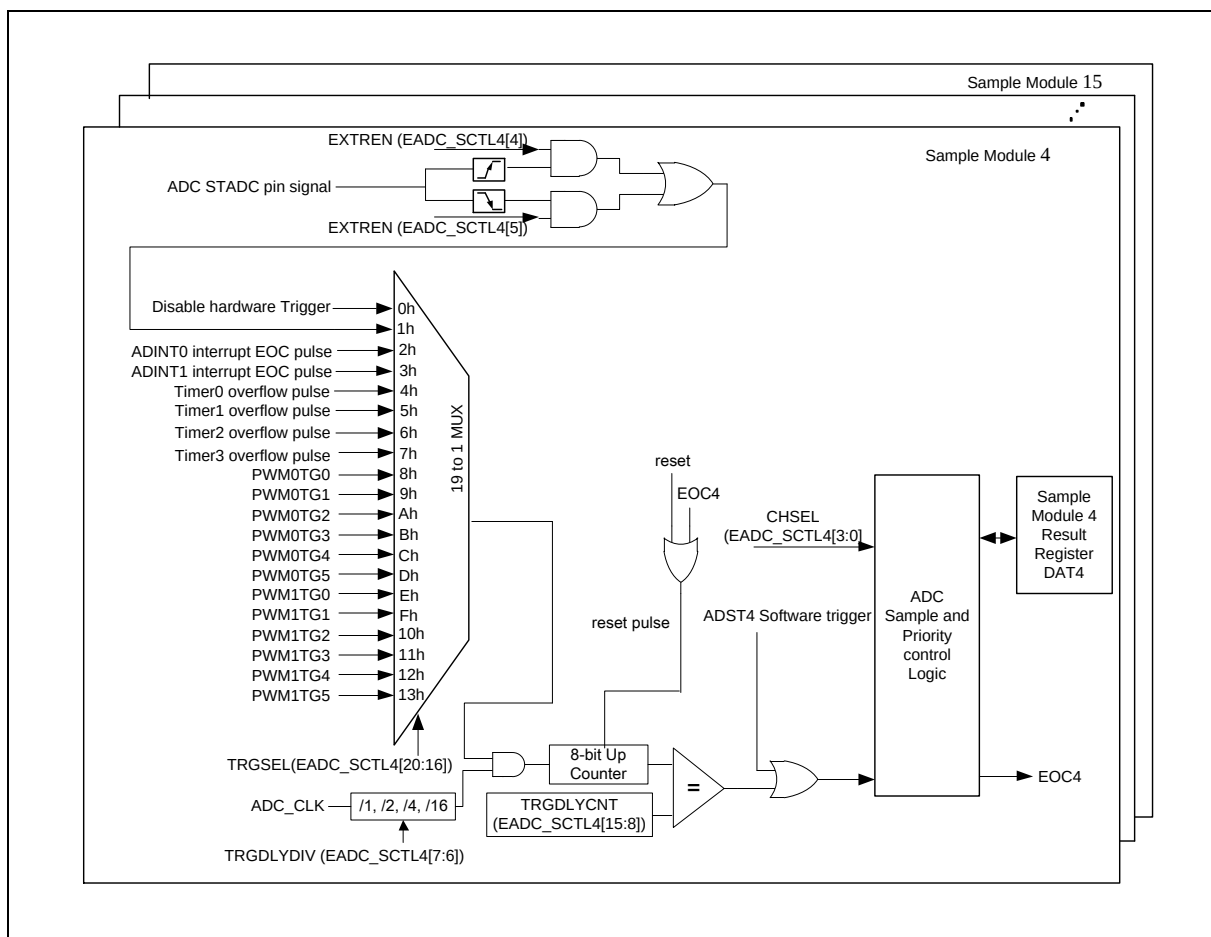
Figure 6.22-3 Sample Module 4~15 Block Diagram
