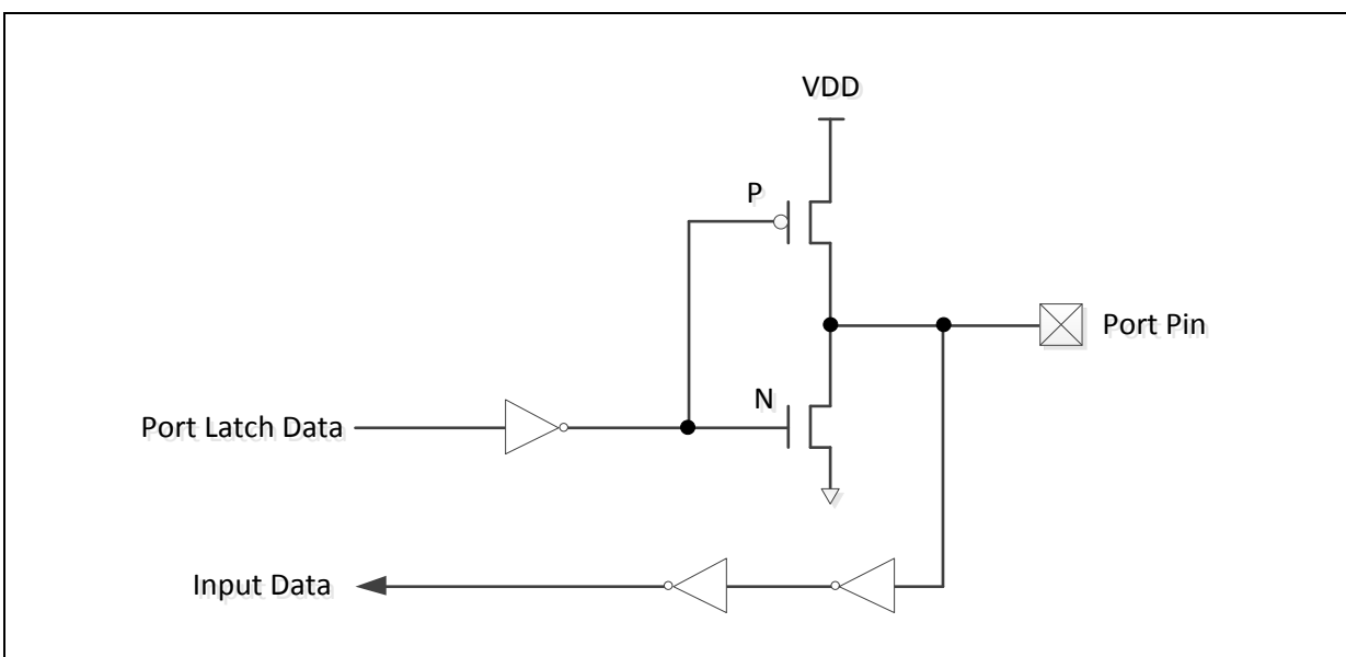
Figure 6.6-2 Push-Pull Output
