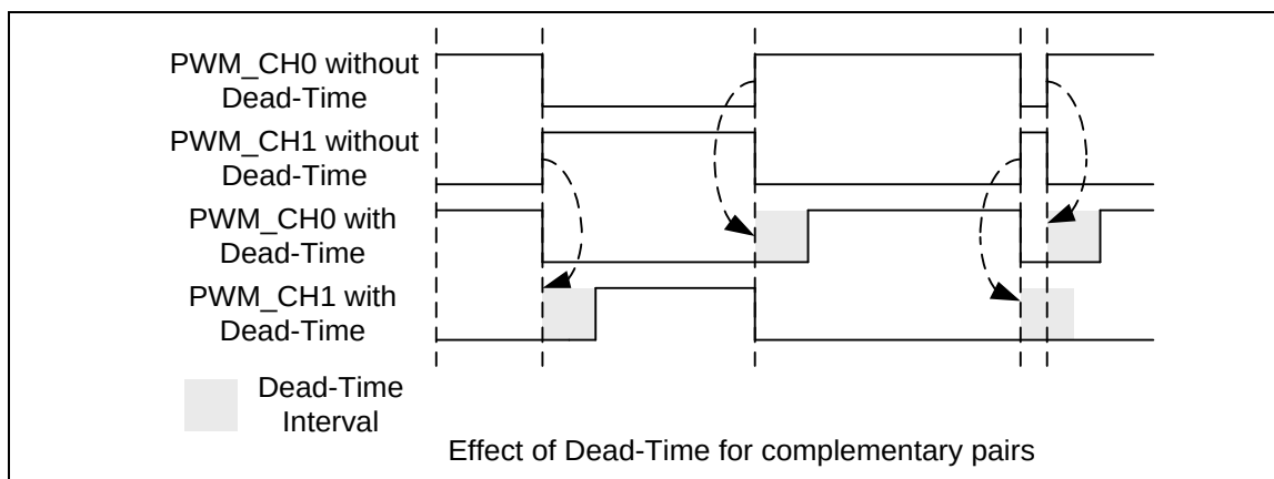
Figure 6.9-27 Dead-Time Insertion
