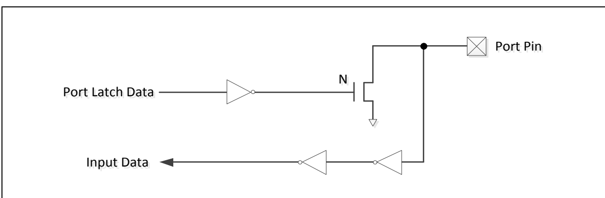
Figure 6.6-3 Open-Drain Output
