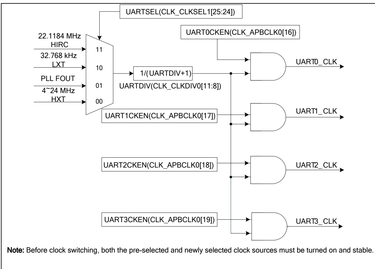
Figure 6.13-1 UART Clock Control Diagram
