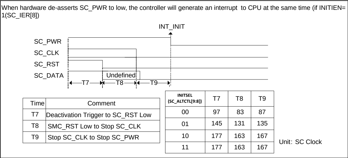
Figure 6.14-6 SC Deactivation Sequence
