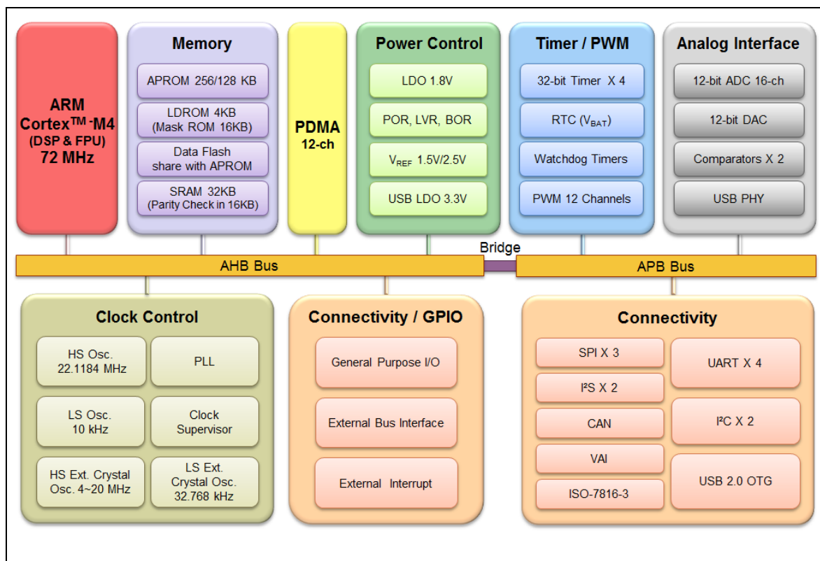
Figure 5.1-1 NuMicro® M45xG/M45xE Block Diagram
