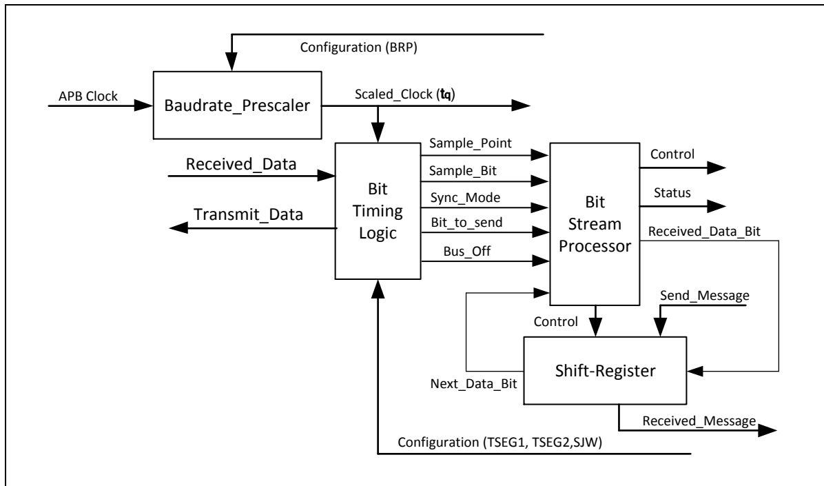
Figure 6.20-11 Structure of the CAN Core's CAN Protocol Controller
