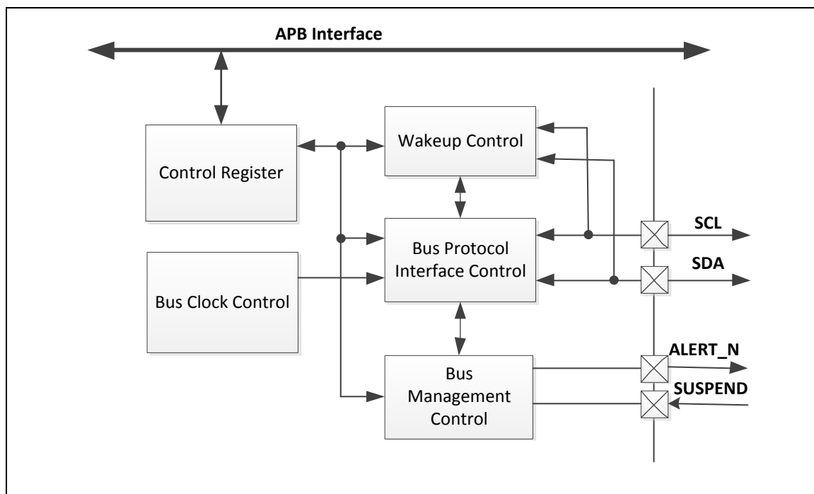
Figure 6.15-1 I 2 C Controller Block Diagram
