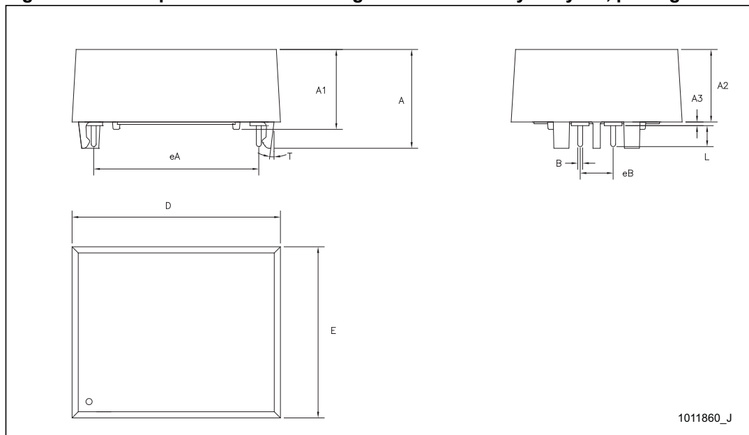
Figure 20. SH – 4-pin SNAPHAT® housing for 48 mAh battery &amp; crystal, package outline
