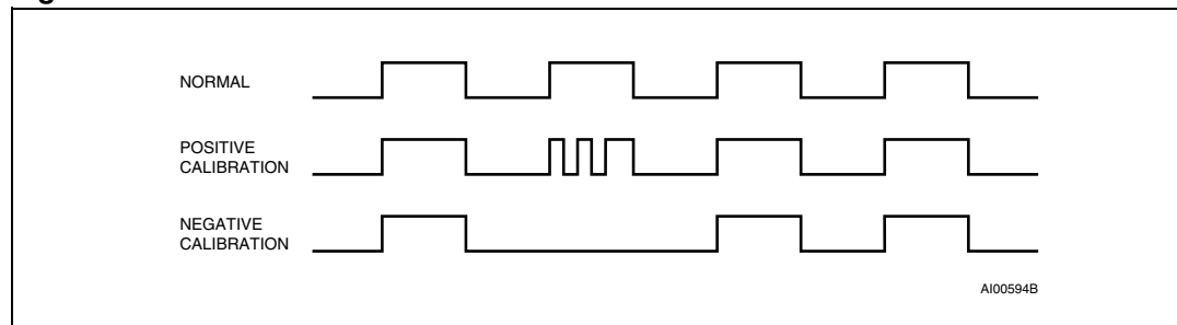
Figure 12. Clock calibration
