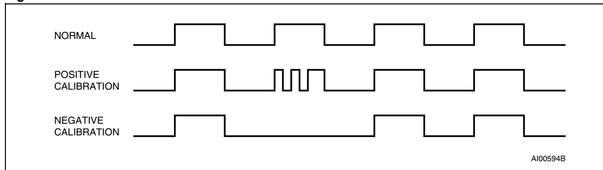
Figure 11. Clock calibration
