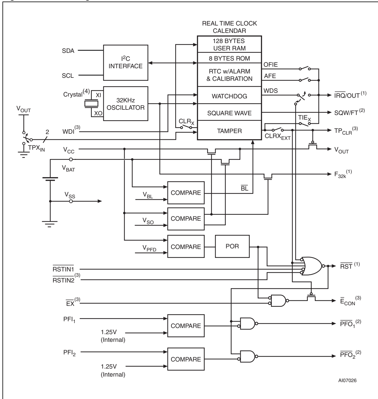
Figure 4. Block diagram
