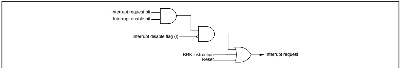
Fig. 13 Interrupt control
