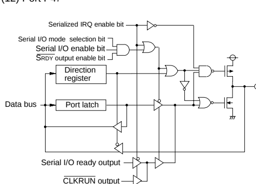
(12) Port P47
