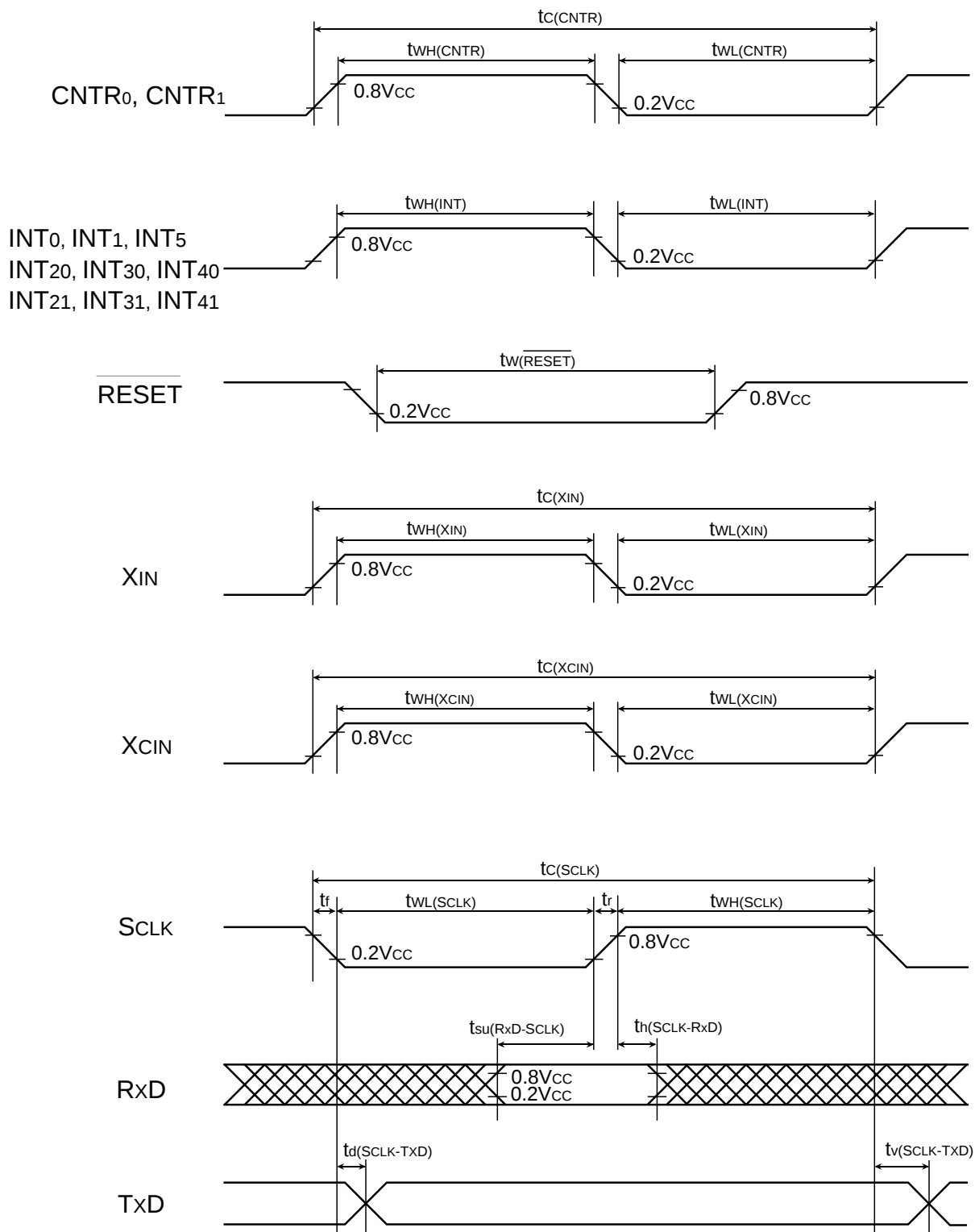
Fig. 84 Timing diagram
