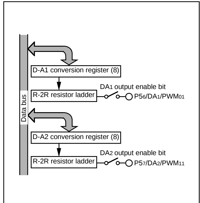
Fig. 62 Block diagram of D-A converter
