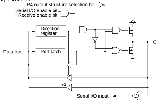
(9) Port P44
