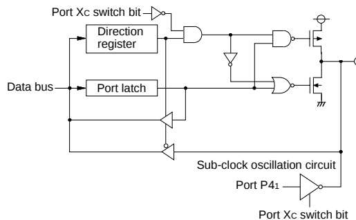
(6) Port P4 0
