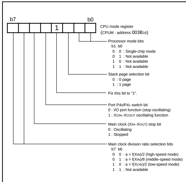
Fig. 7 Structure of CPU mode register
