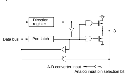
(16) Port P6
