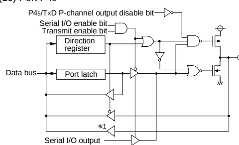
(10) Port P45
