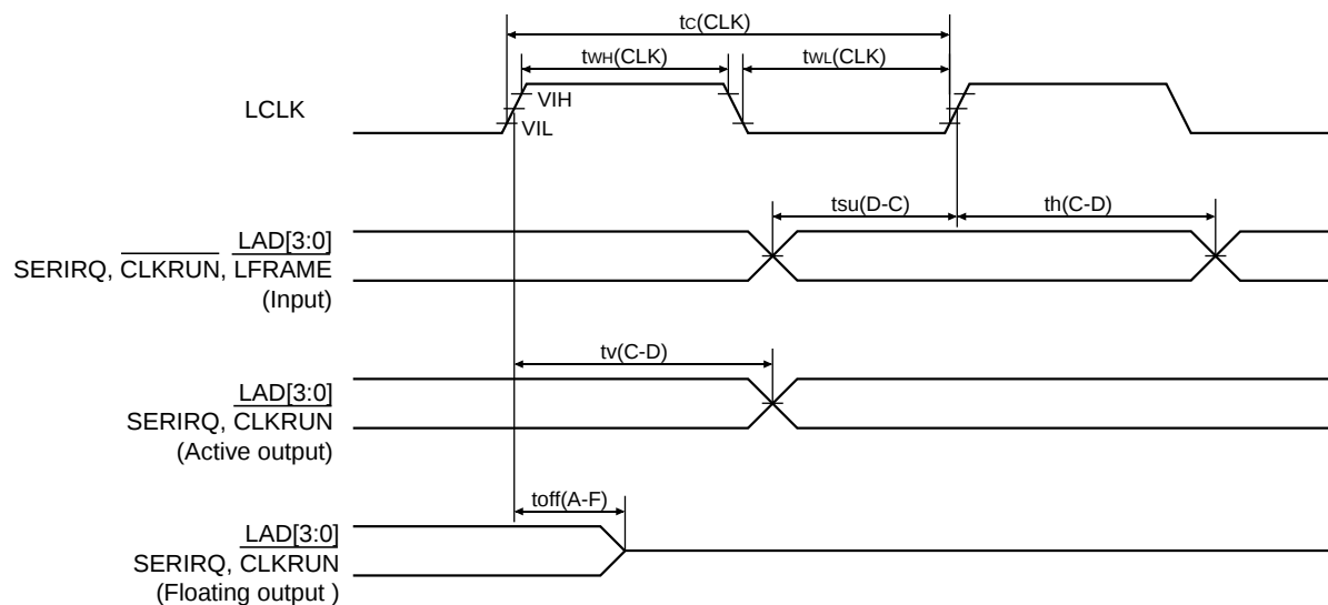
Fig. 86 Timing diagram of LPC Interface and Serialized IRQ
