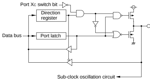
(7) Port P4 1
