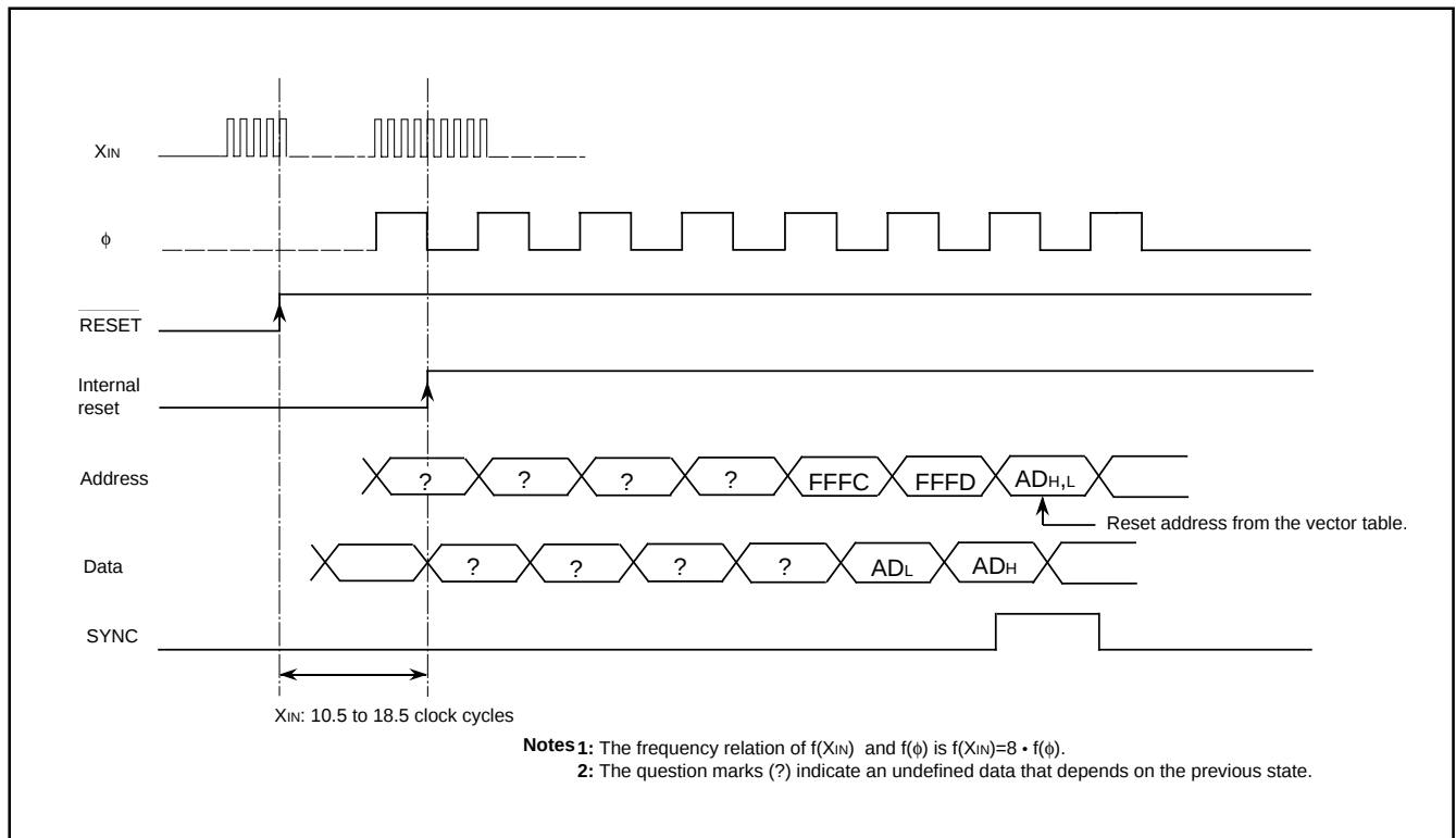
Fig. 66 Reset sequence
