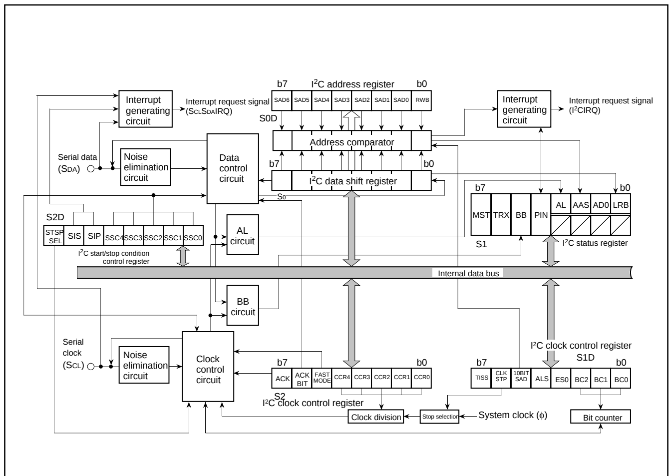
Fig. 31 Block diagram of multi-master I 2 C-BUS interface
