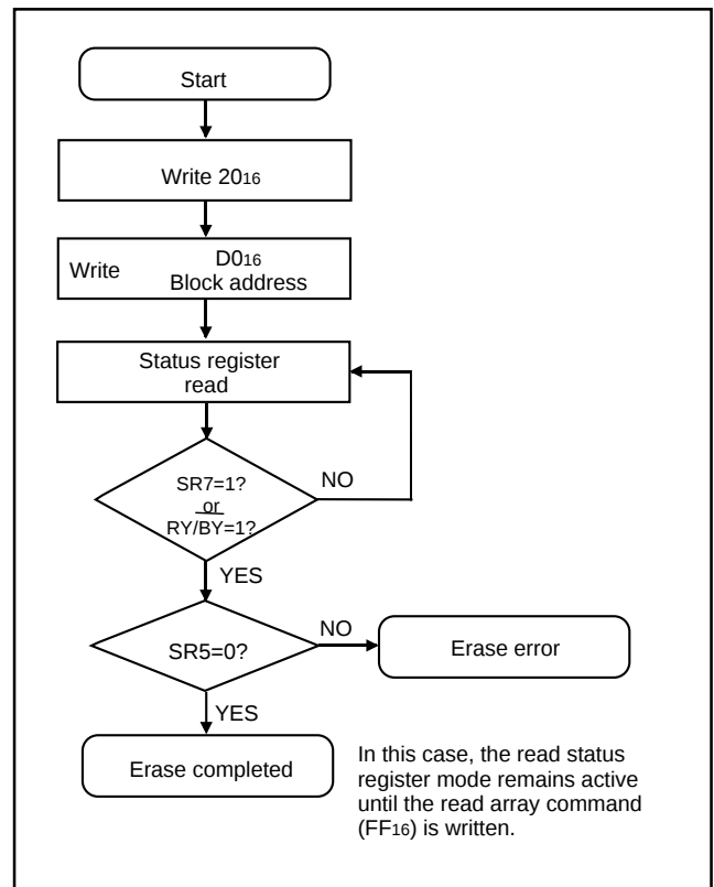
Fig. 75 Block erase flowchart
