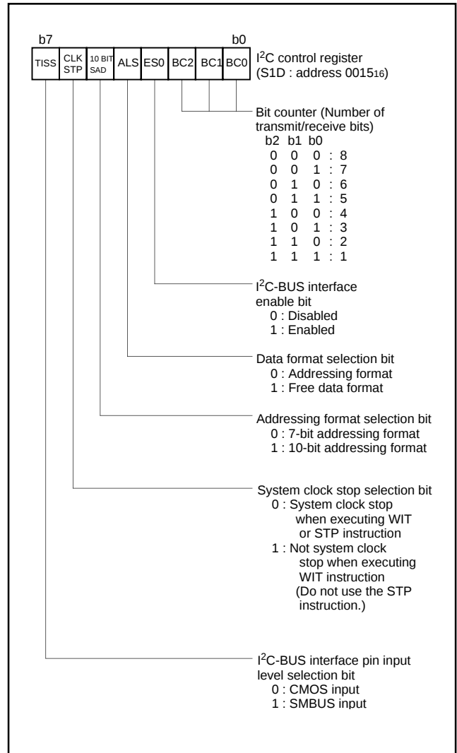
Fig. 34 Structure of I 2 C control register
