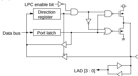
(14) Ports P80 to P83
