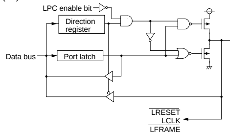
(15) Ports P84 to P86
