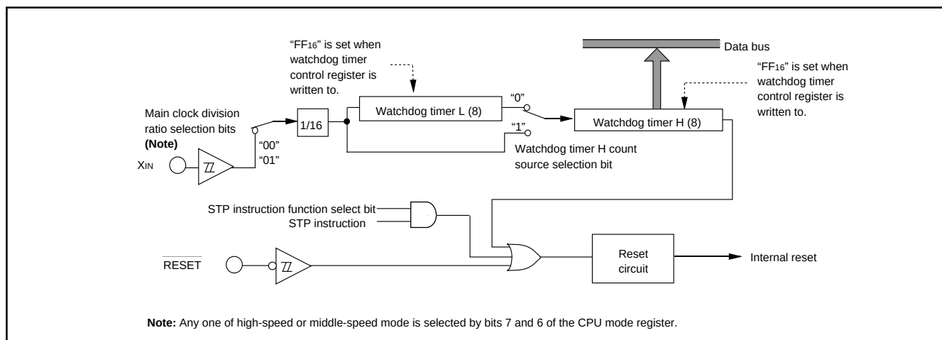
Fig. 21 Block diagram of Watchdog timer
