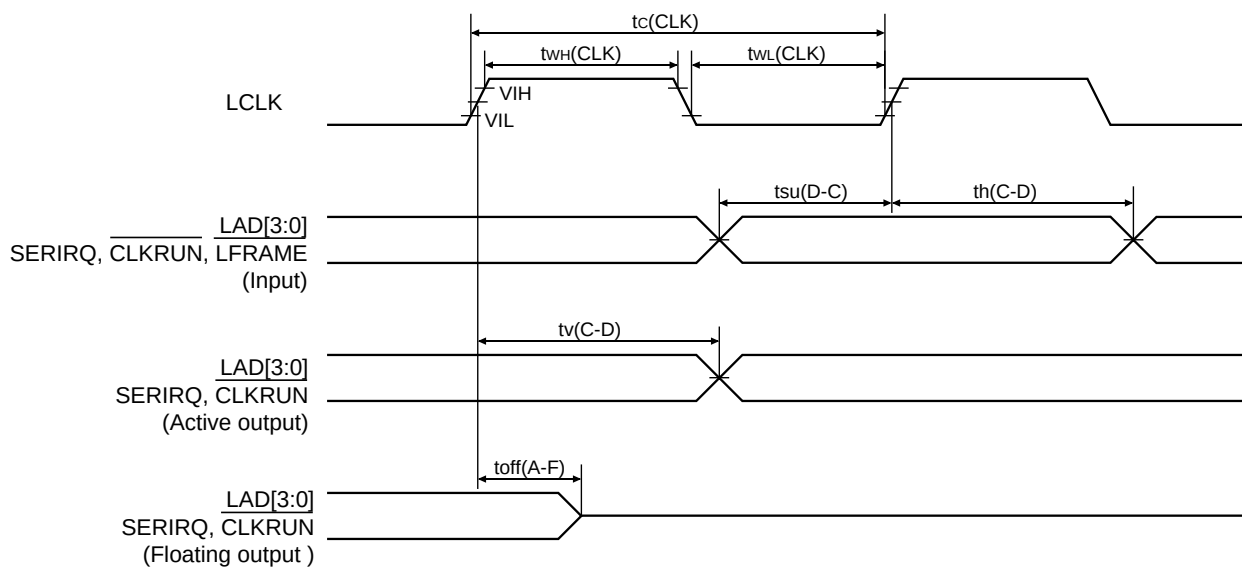
Timing diagrams of LPC Bus Interface and Serial Interrupt Output
