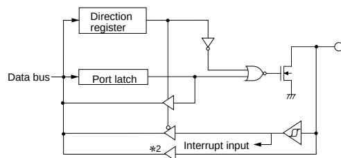
(12) Ports P73 to P75
