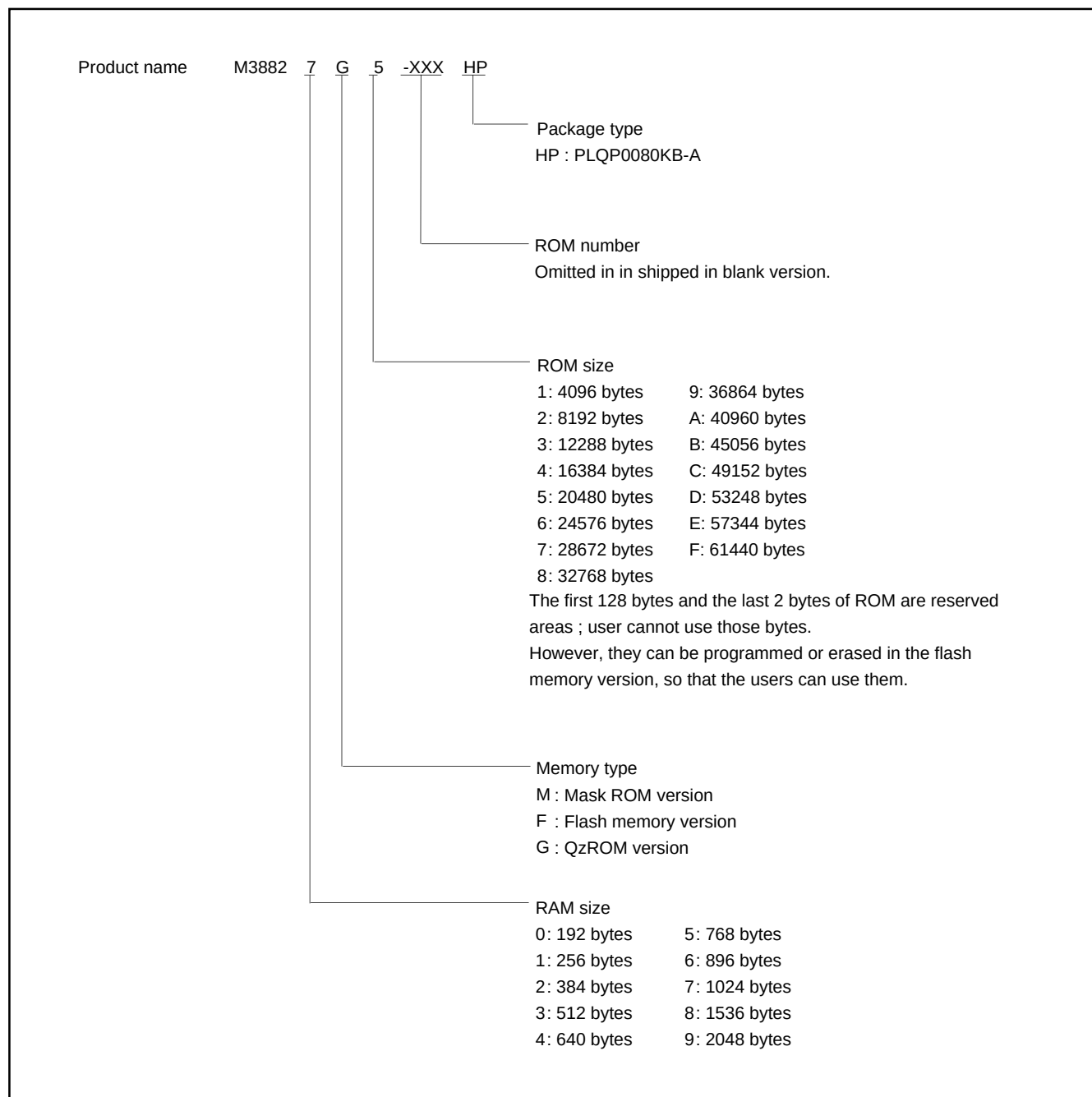
Fig. 3 Part numbering
