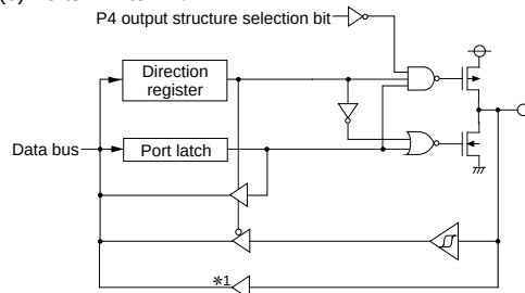
(6) Ports P44 to P46
