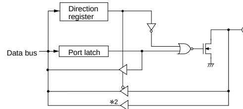
(13) Port P76, P77
