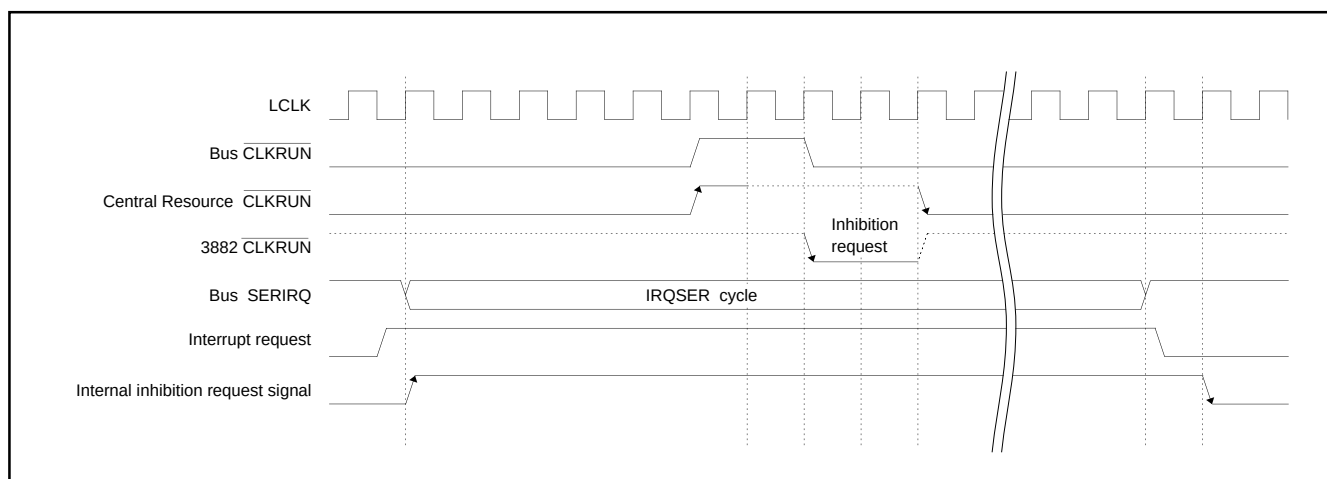
Fig. 38 Timing diagram of clock stop inhibition request
