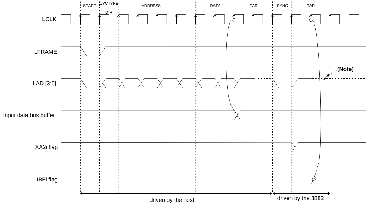
Fig. 28 Data and command write timing
