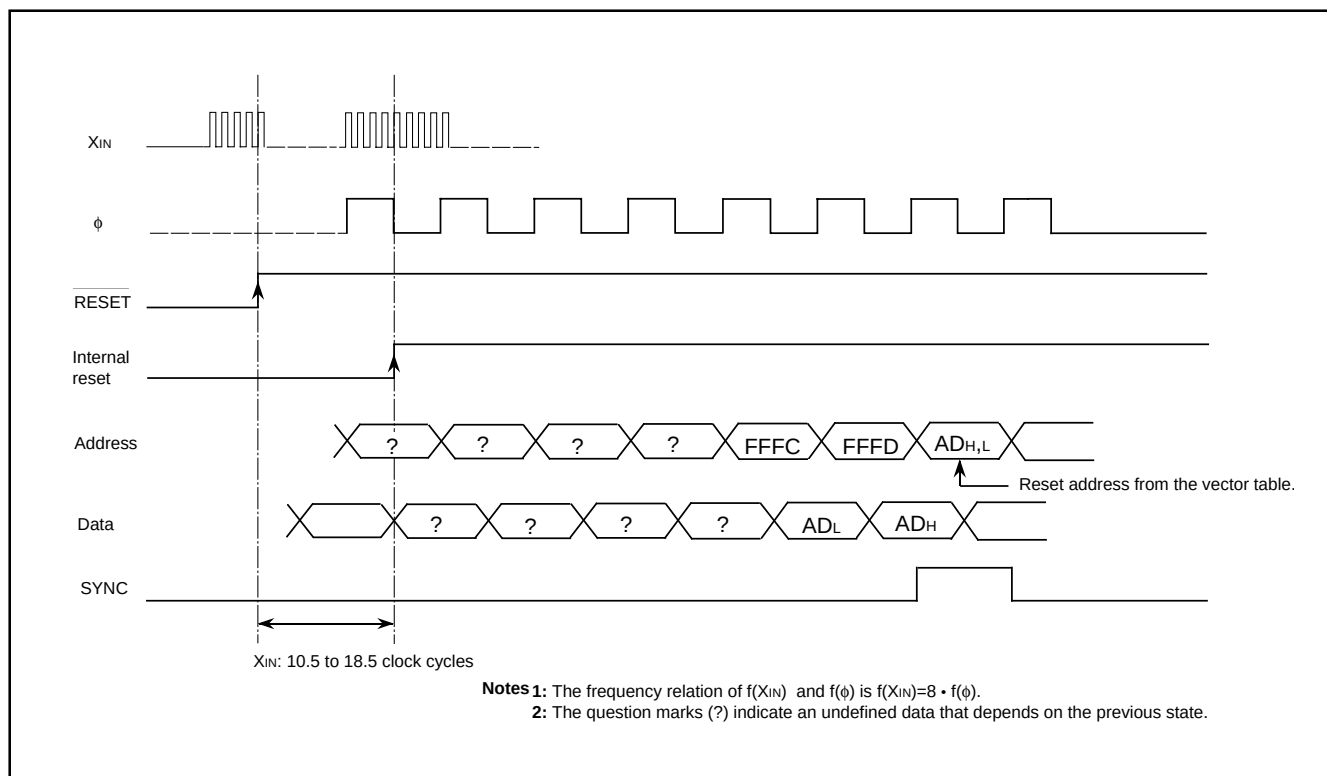
Fig. 40 Reset sequence
