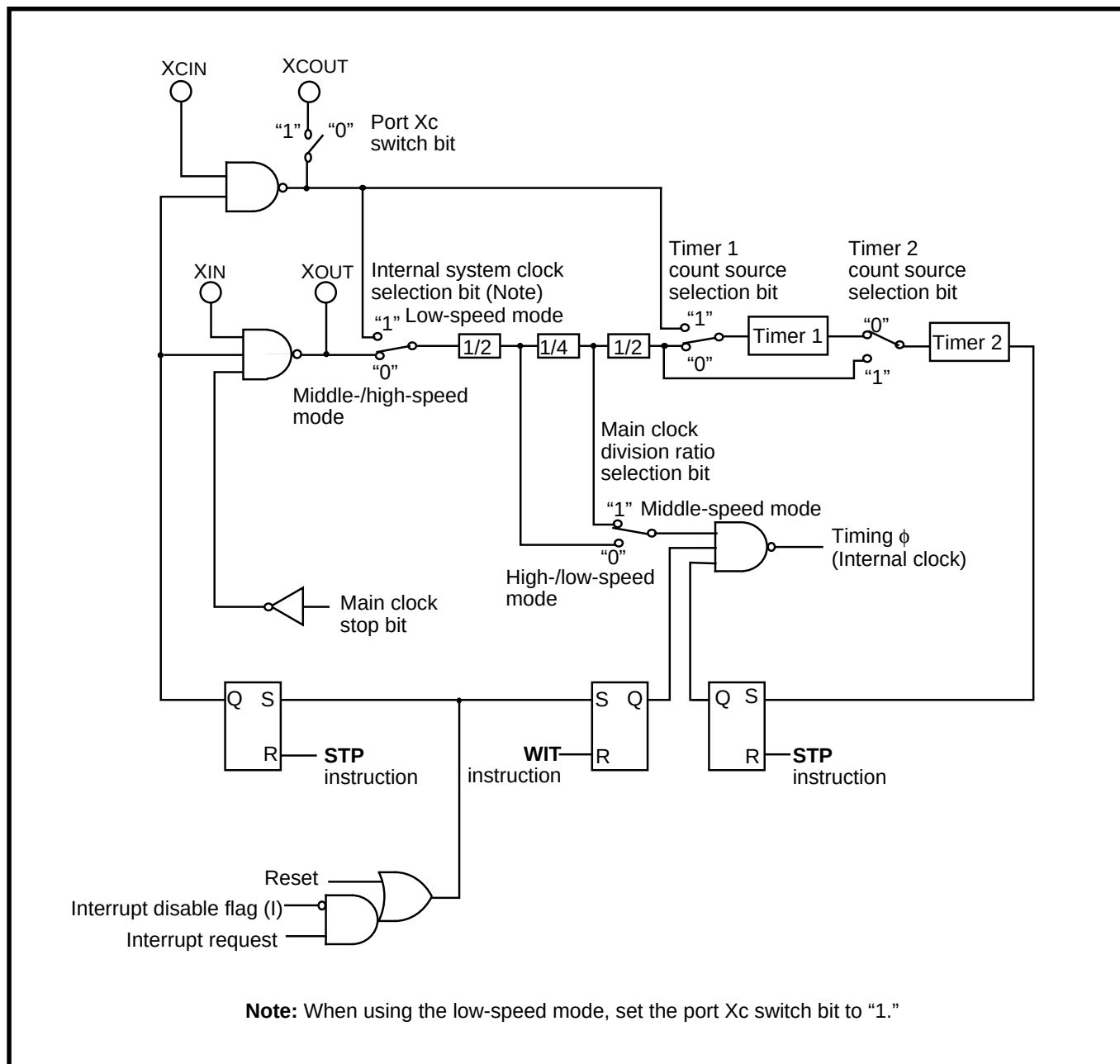
Fig. 2.11.3 Clock generating circuit block diagram
