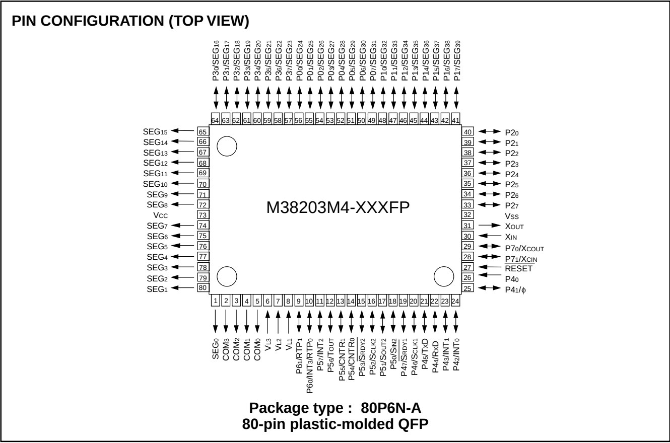
Pin configuration of M38203M4-XXXXFP
