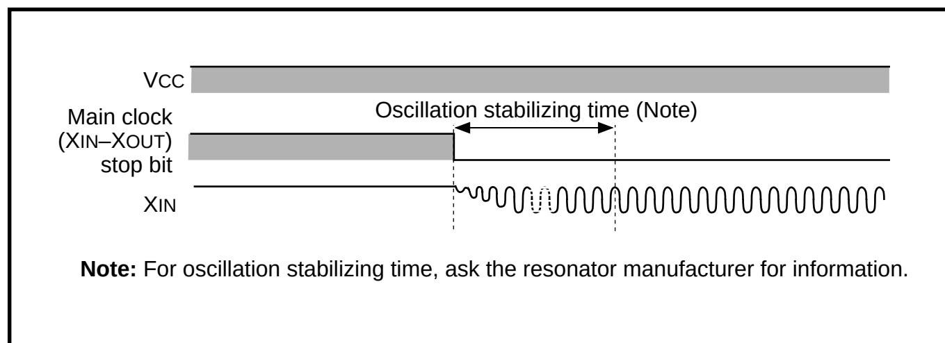
Fig. 2.11.7 Oscillation stabilizing time at reoscillation of X IN
