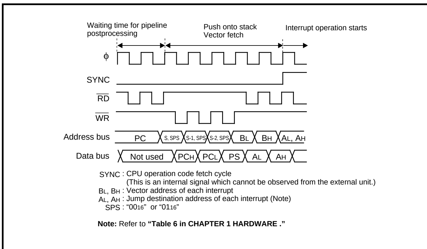
Fig. 2.2.4 Timing after acceptance of interrupt request
