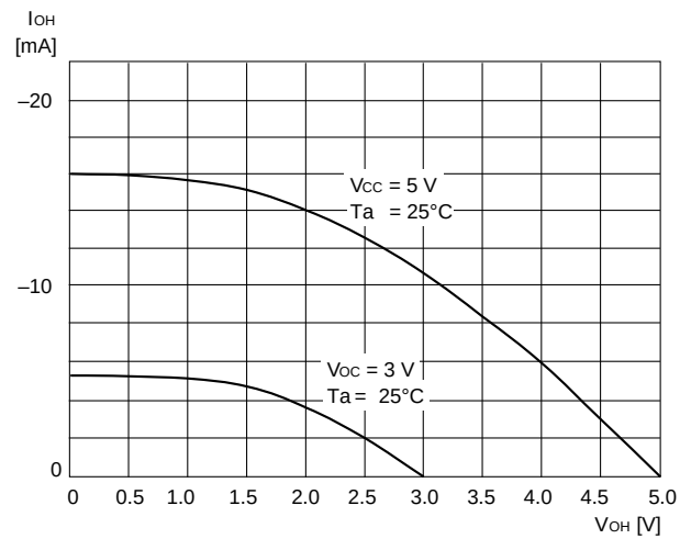
Port P0 0 I OH -V OH characteristic (P-channel drive) (Pins with same characteristic : P0, P1, P3)
