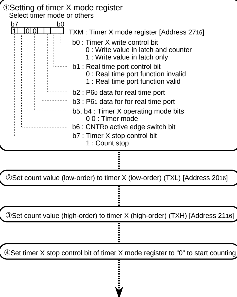
Fig. 2.3.23 Example of setting registers for using timer mode
