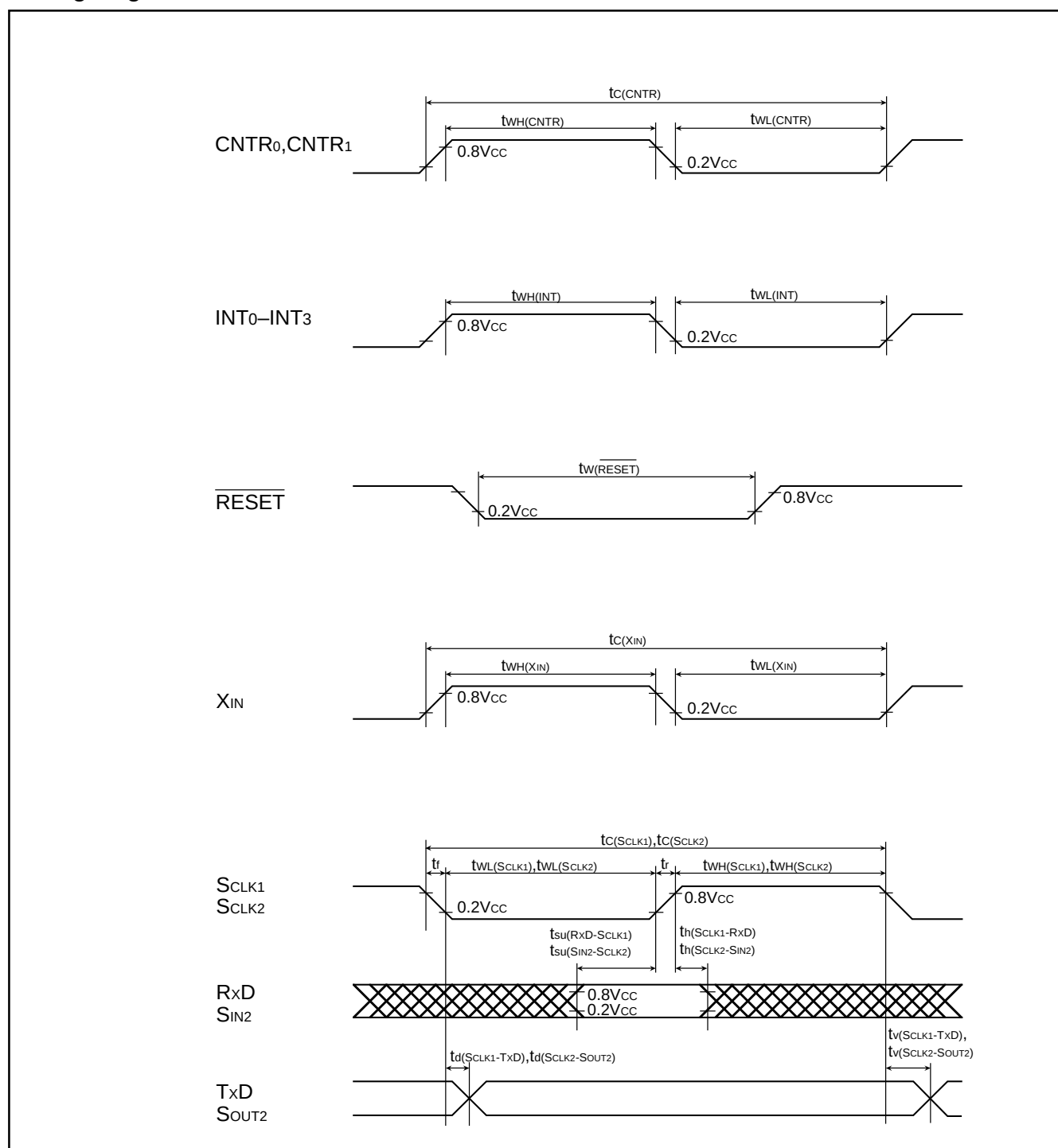
Fig.48 Timing diagram
