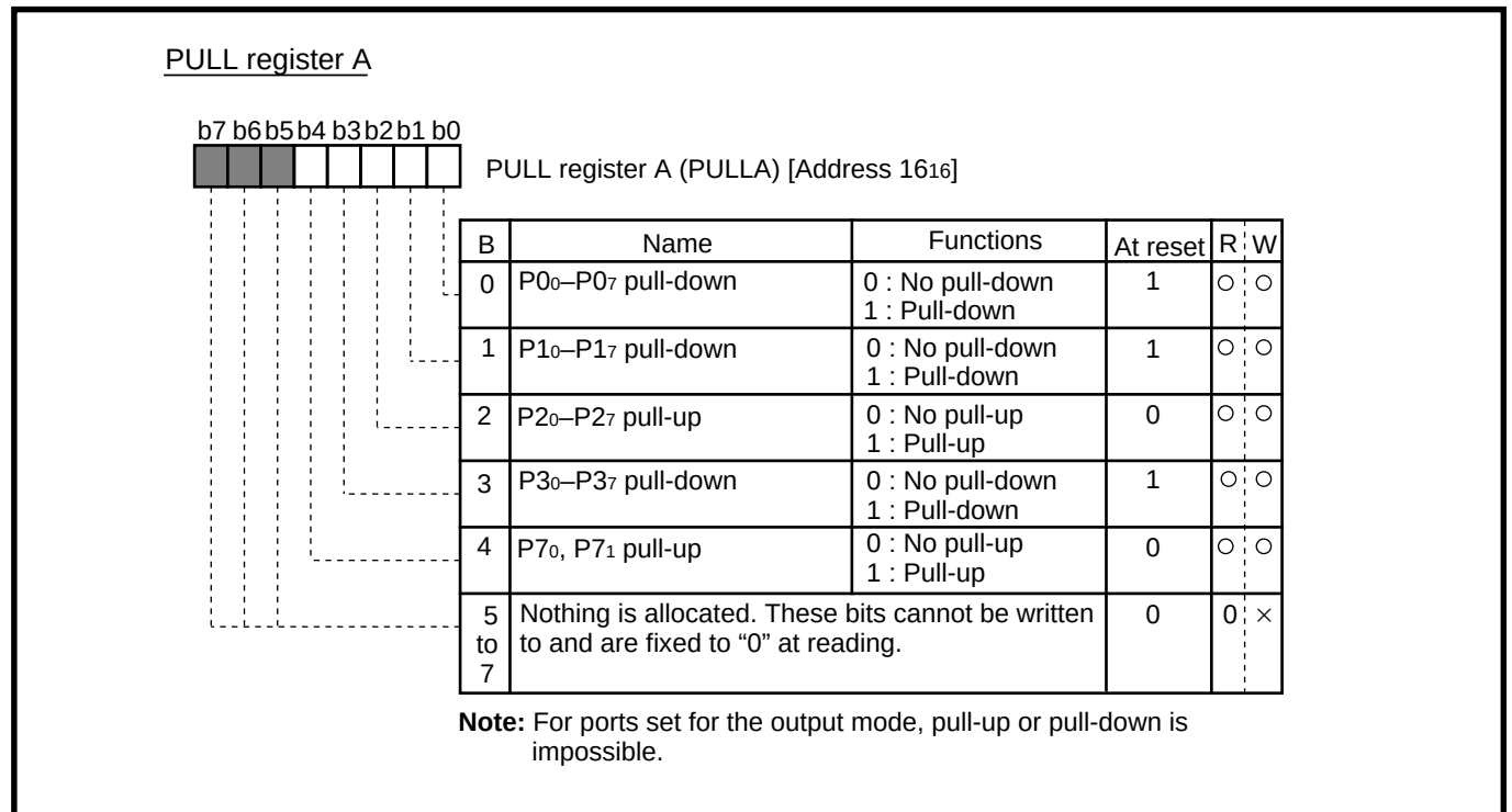
Fig. 2.1.5 Structure of PULL register A
