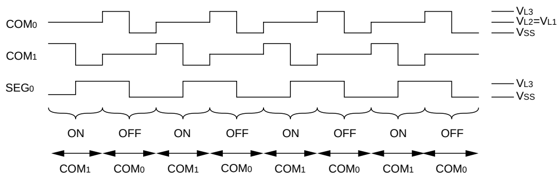
Fig. 34 LCD drive waveform (1/2 bias)
