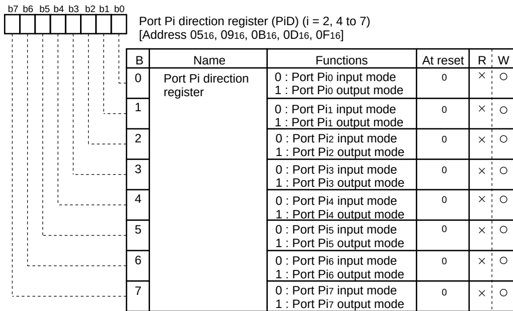
Port Pi direction register
