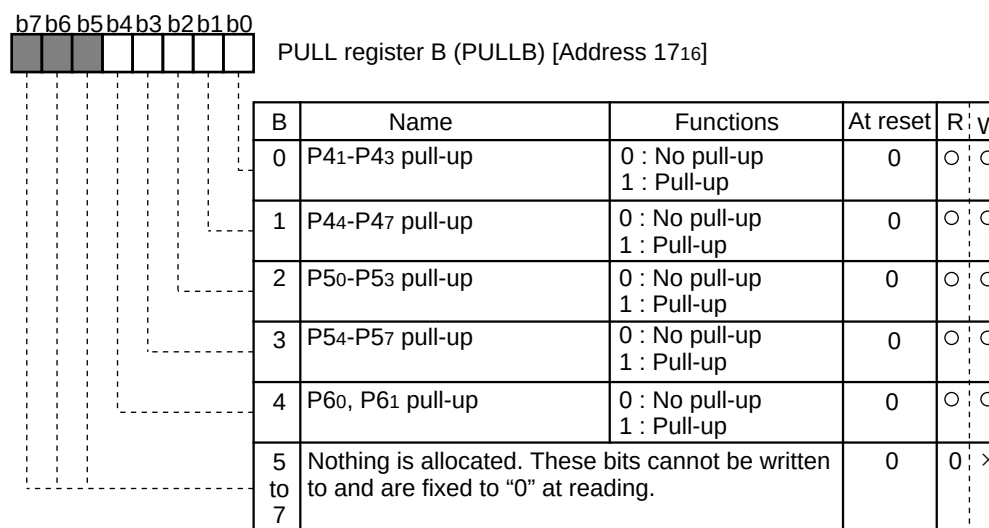
PULL register B
