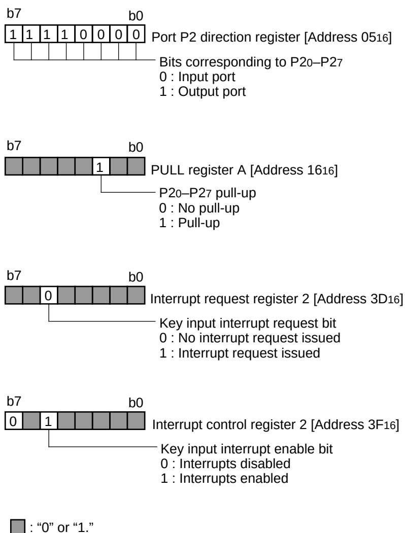
Fig. 2.2.16 Setting values (corresponding to Figure 2.2.15) of key input interrupt-related registers
