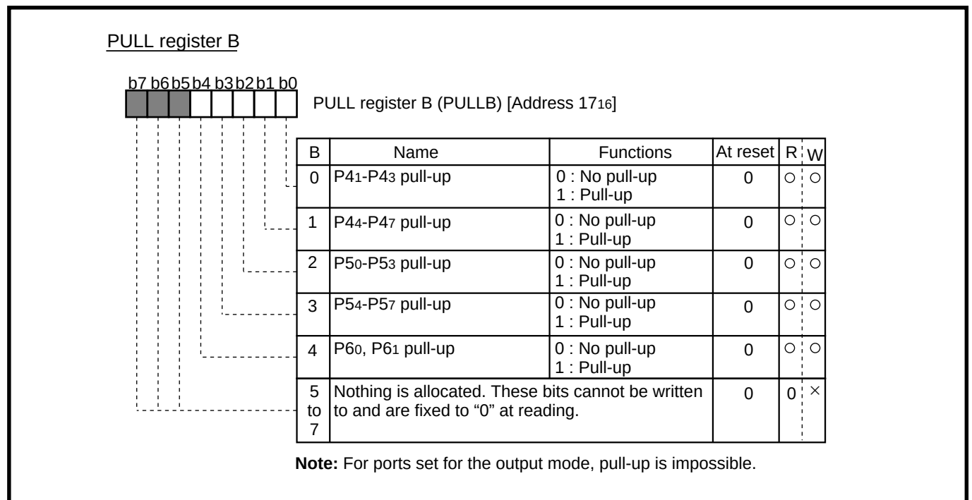
Fig. 2.1.6 Structure of PULL register B
