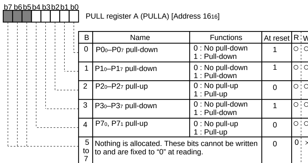
PULL register A
