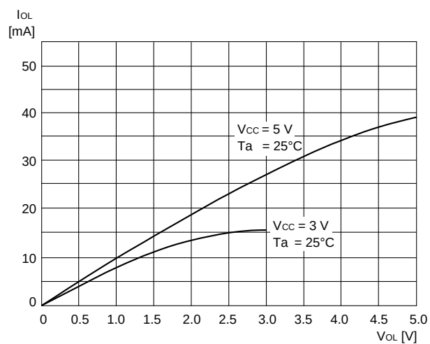
Port P0 0 I OL -V OL characteristic (N-channel drive) (Pins with same characteristic : P0, P1, P3)
