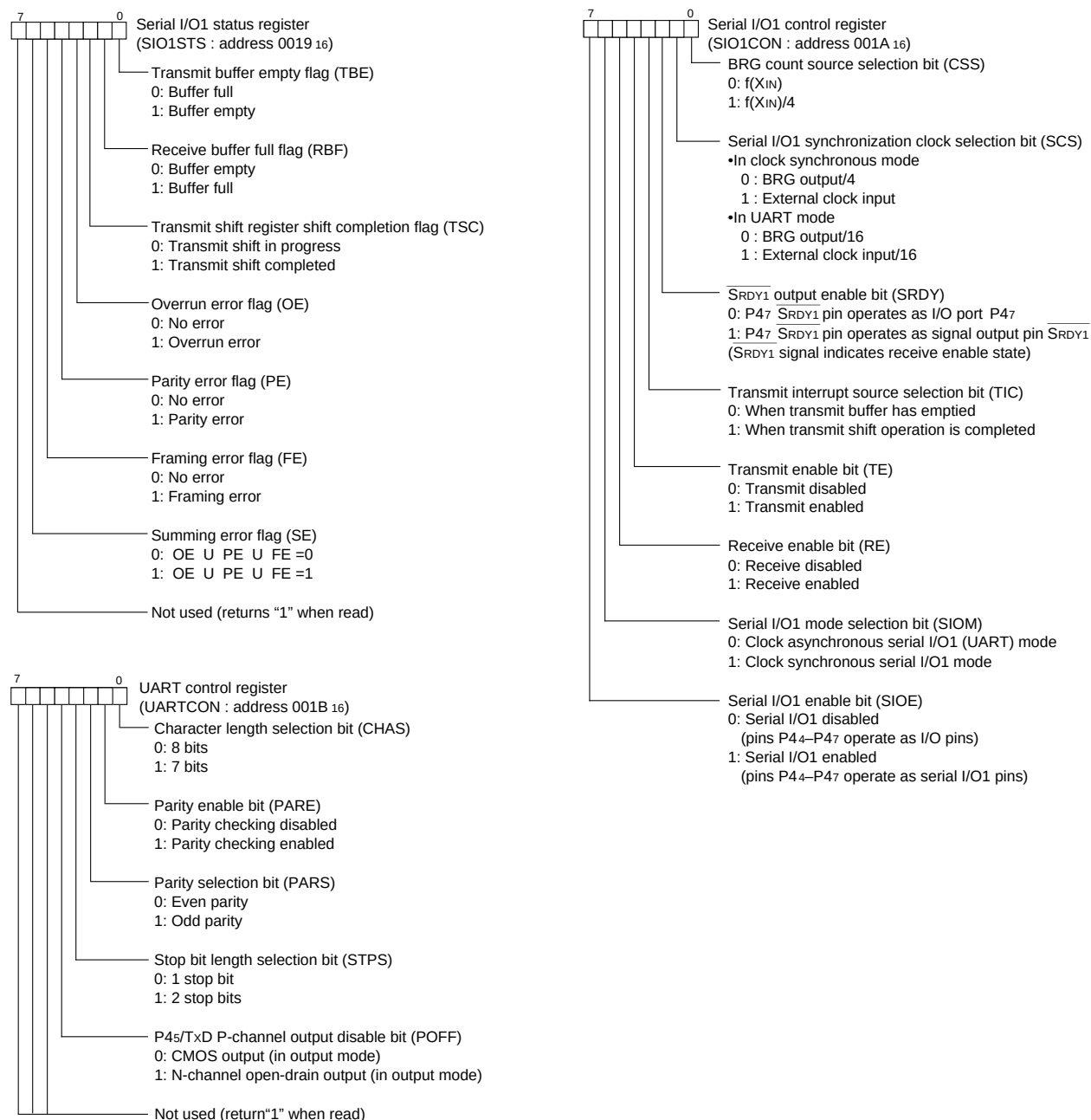
Fig. 26 Structure of serial I/O1 control registers
