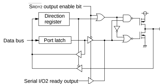
(4) Port P03
