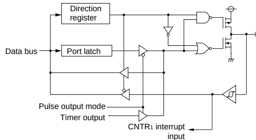
(14) Port P40
