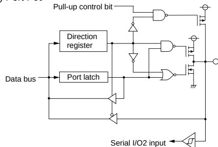
(1) Port P00
