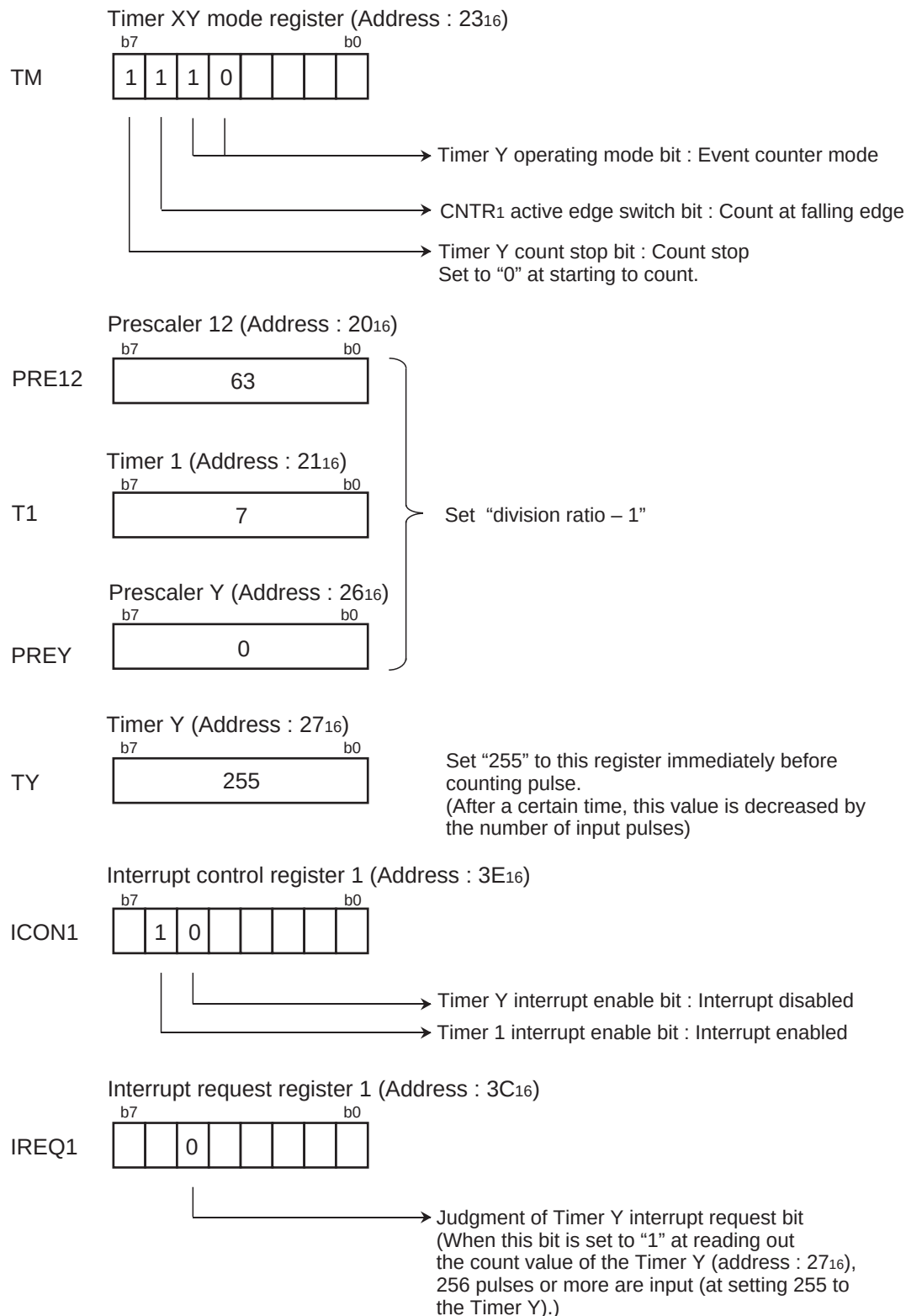
Fig. 2.2.18 Setting of related registers [Measurement of frequency]
