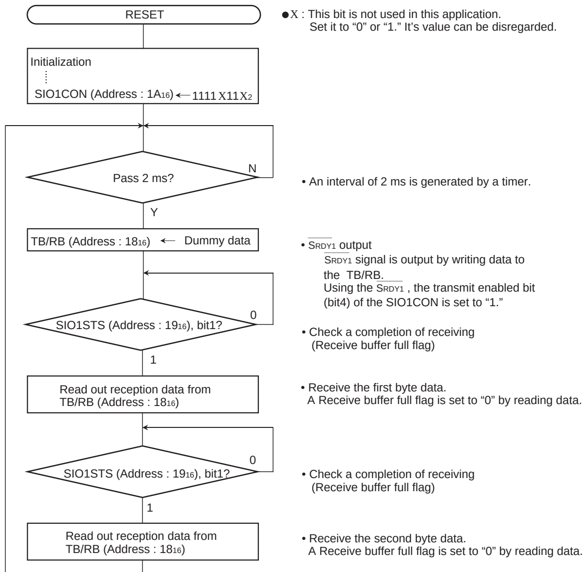
Fig. 2.3.22 Control procedure at a receiving side [Communication using a clock synchronous serial I/O]
