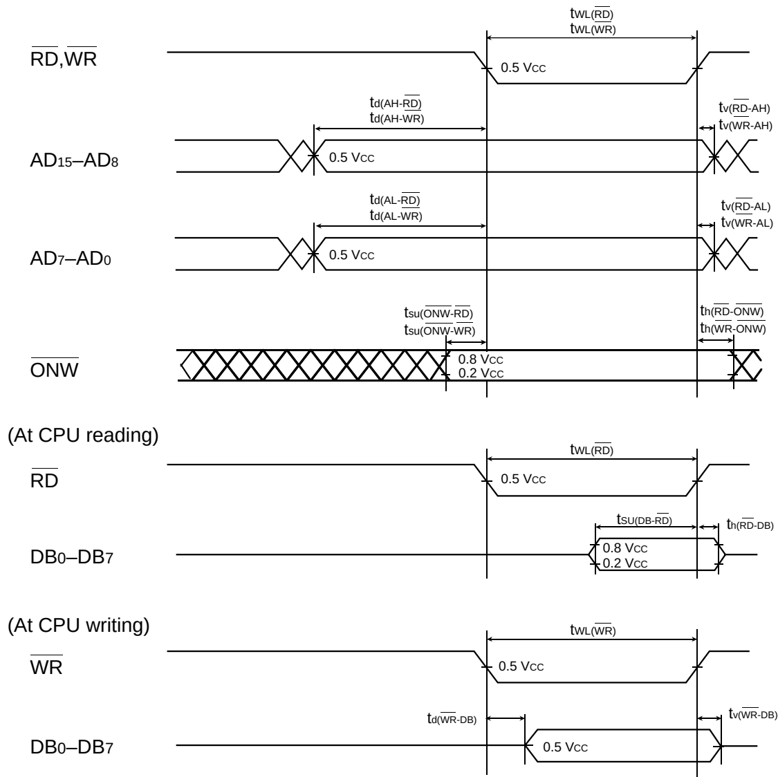
Fig. 3.1.4 Timing diagram (in memory expansion mode and microprocessor mode) (2)
