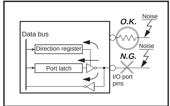
Fig. 3.4.8 Setup for I/O ports
