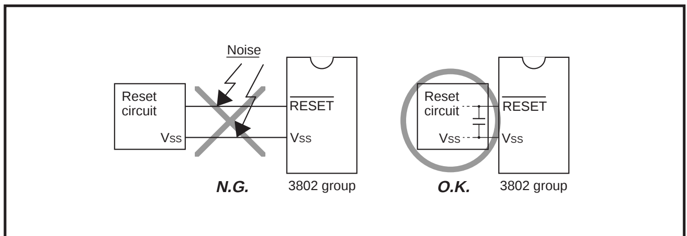
Fig. 3.4.1 Wiring for the RESET pin
