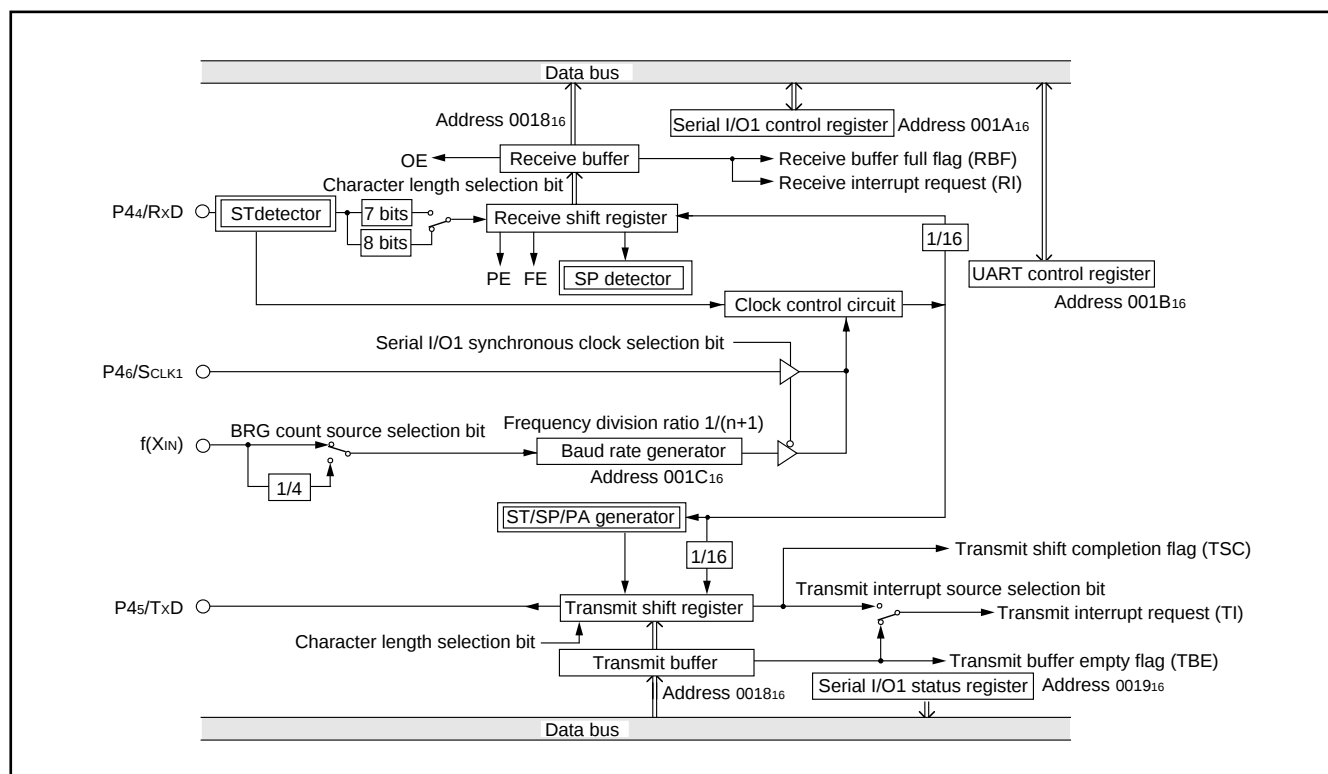
Fig. 20 Block diagram of UART serial I/O
