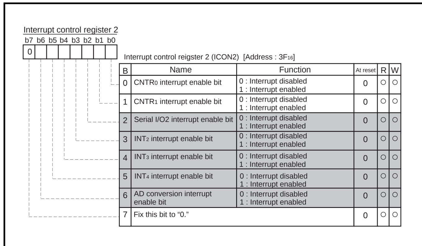
Fig. 2.2.9 Structure of Interrupt control register 2
