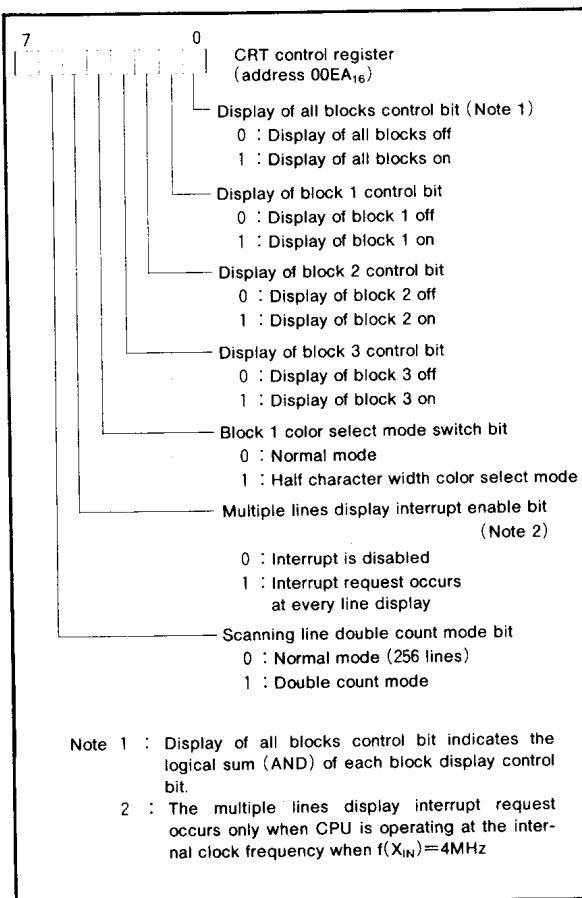
Fig. 22 Structure of CRT control register
