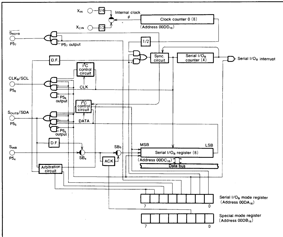
Fig. 11 Block diagram of serial I/O B
