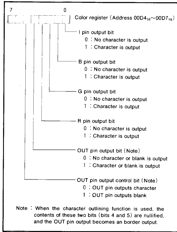
Fig. 29 Structure of color registers
