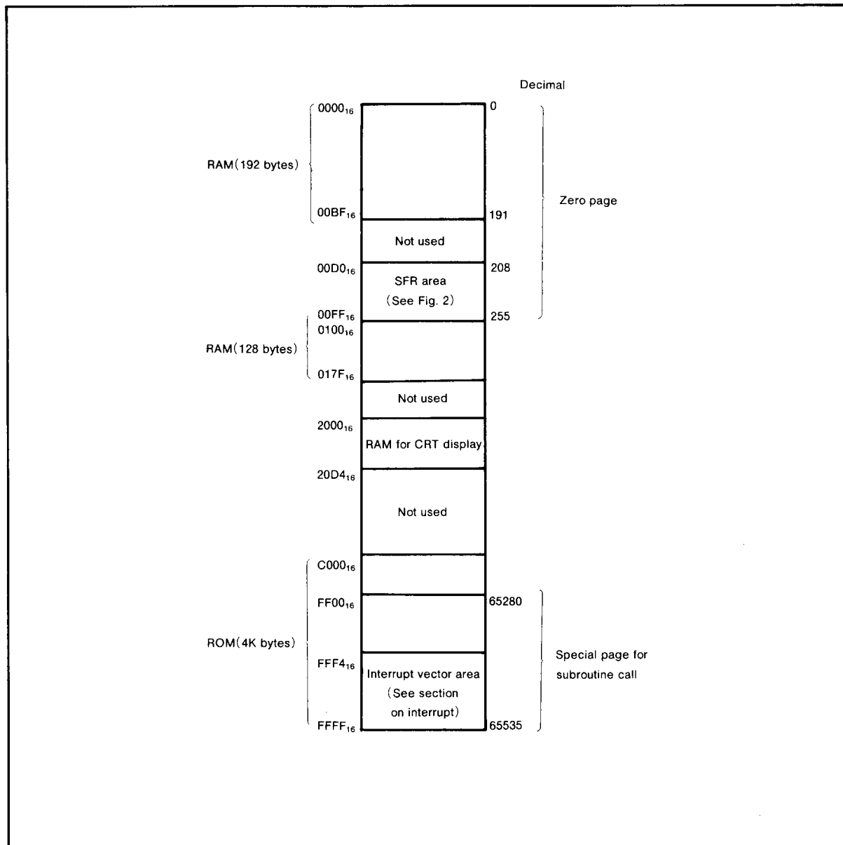
Fig. 1 Memory map
