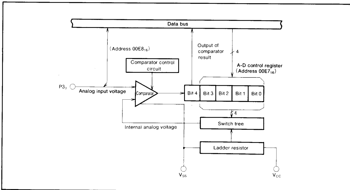
Fig. 20 Comparator Circuit
