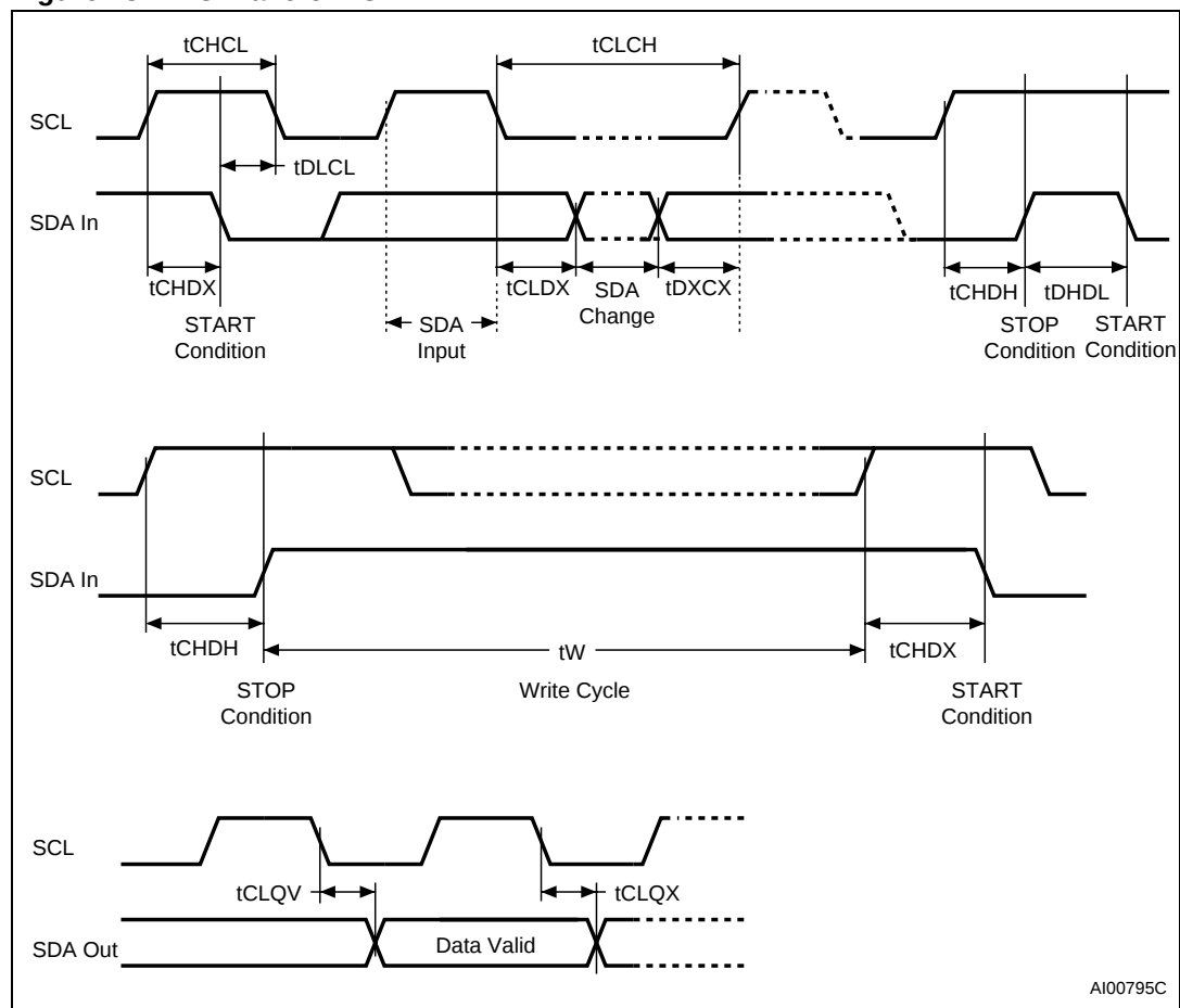
Figure 13. AC Waveforms
