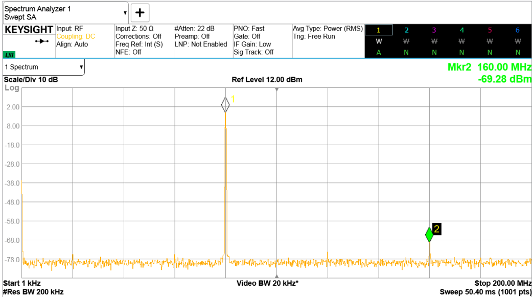
Figure 3. Single-tone spectrum @ f_{out} = 80\text{ MHz}
