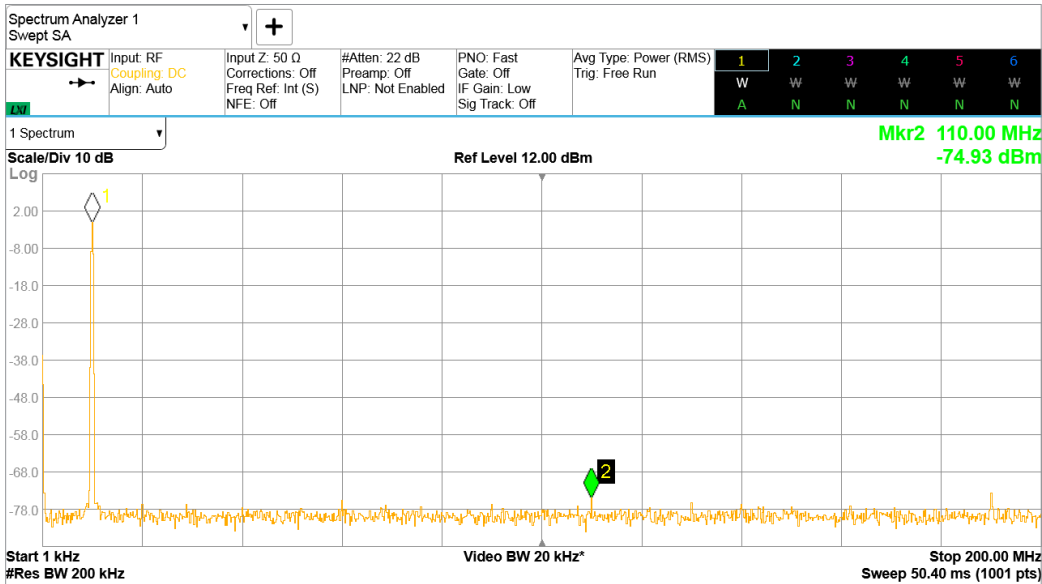
Figure 2. Single-tone spectrum @ f_{out} = 10\text{ MHz}
