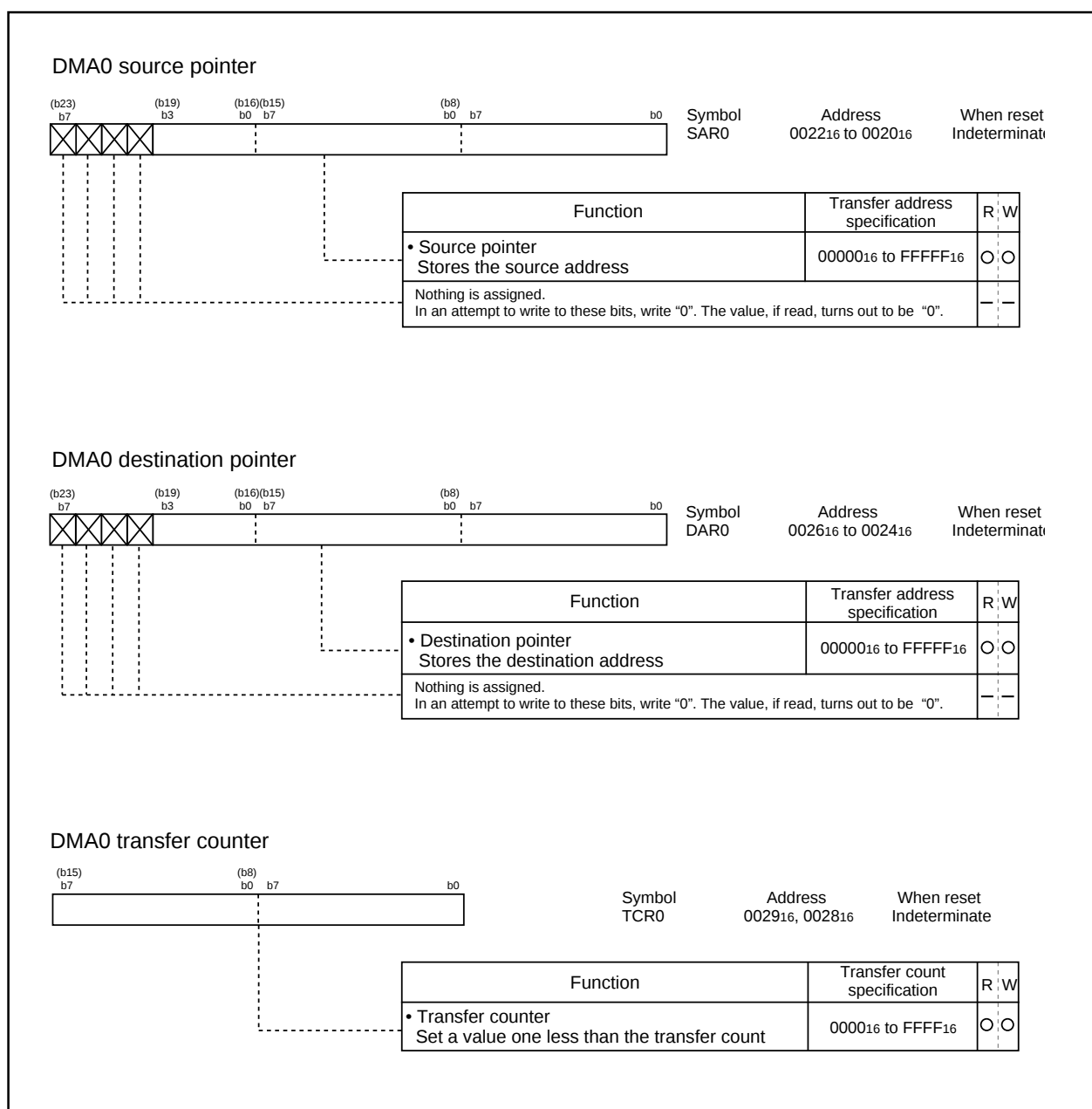
Figure 1.13.4. DMAC register (3)
