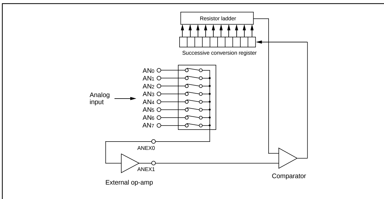
Figure 1.17.5. Example of external op-amp connection mode
