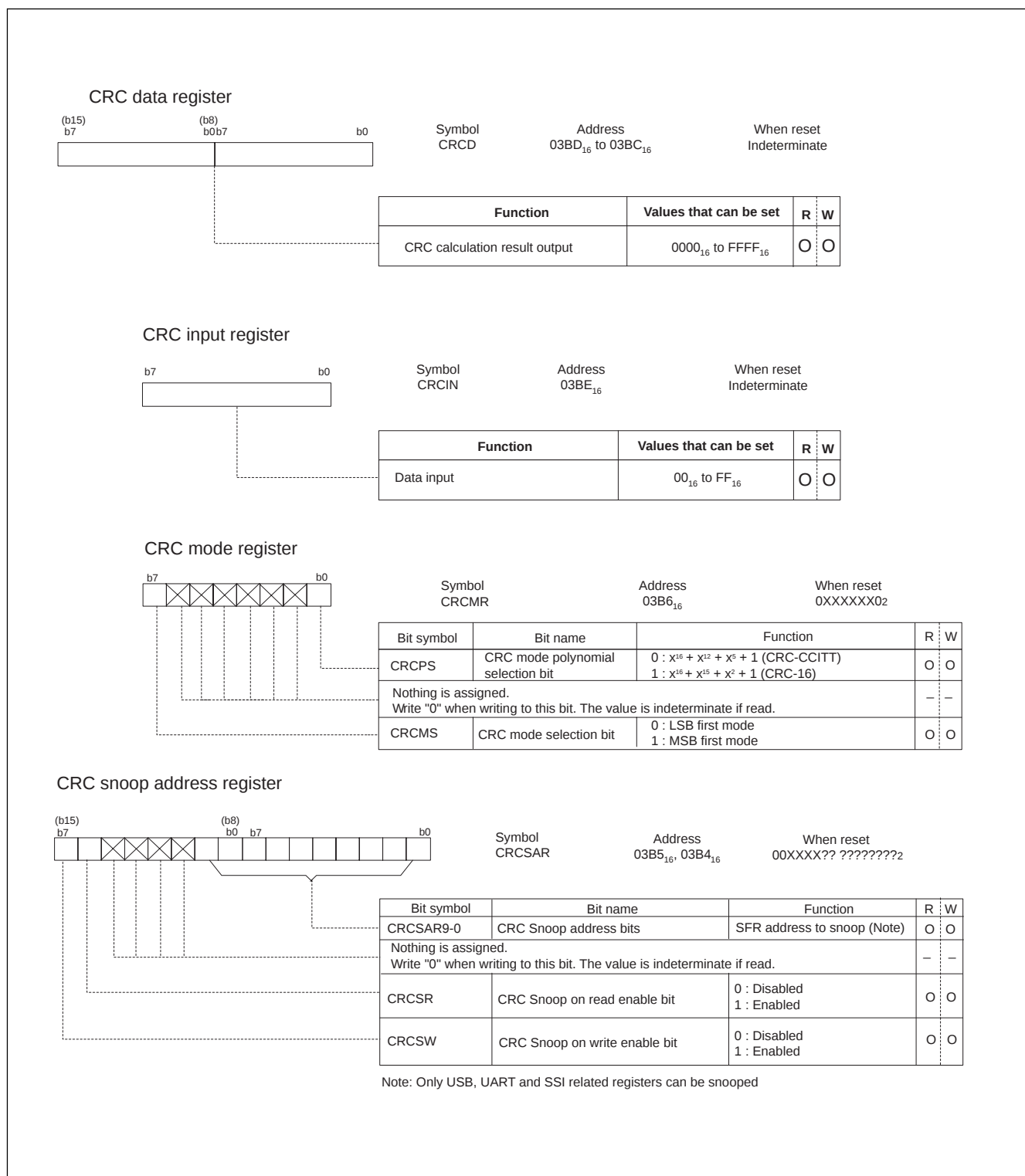
Figure 1.130. CRC-related registers
