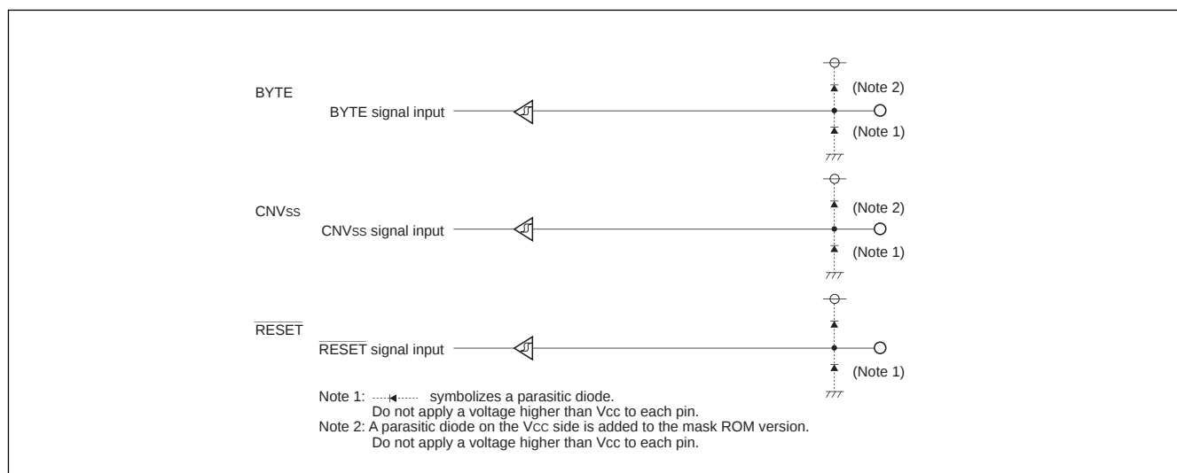
Figure 1.136. I/O pins
