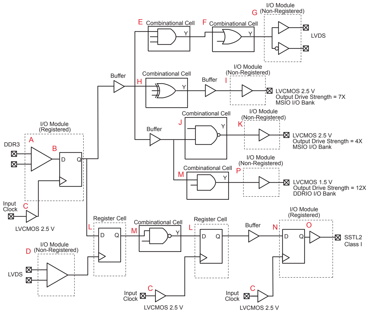
Figure 2-1 • Timing Model
