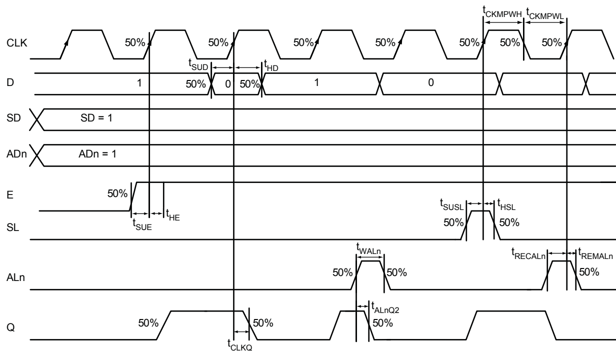
Figure 2-8 • Timing Diagram
