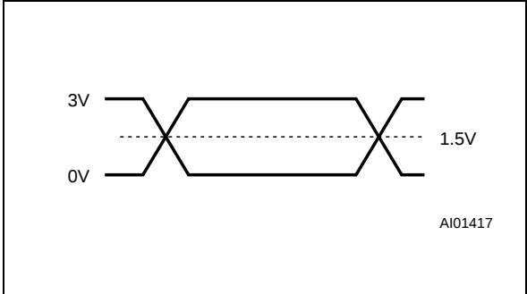
Figure 7. AC Testing Input Output Waveform
