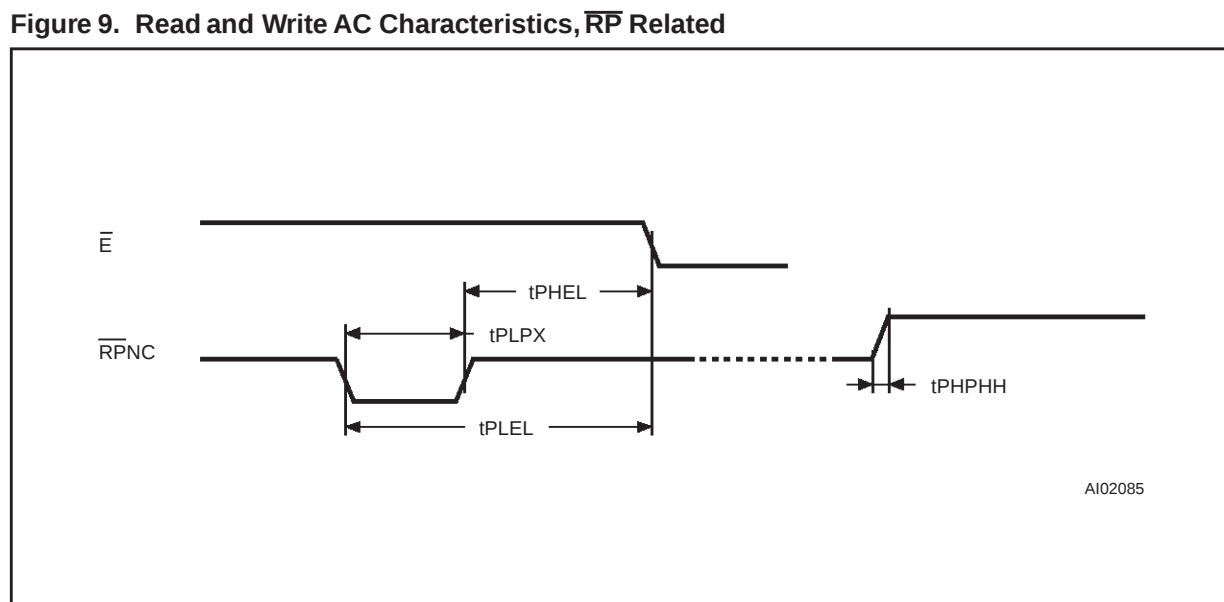
Note: Address are latched on the falling edge of \overline{E} , Data is latched on the rising edge of \overline{E} .
