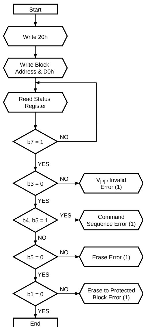
Figure 21. Erase Flowchart and Pseudo Code
