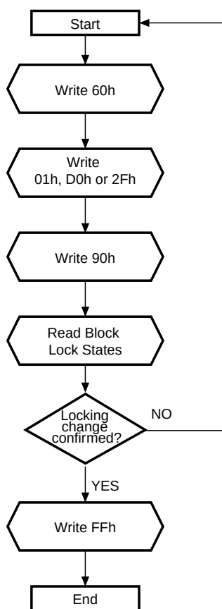
Figure 23. Locking Operations Flowchart and Pseudo Code
