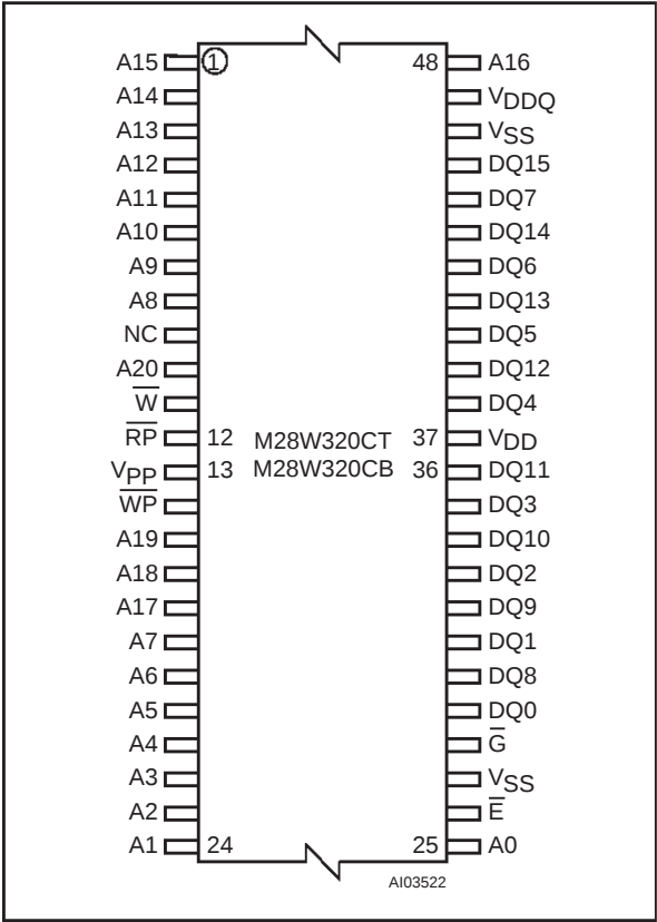
Figure 3. TSOP Connections
