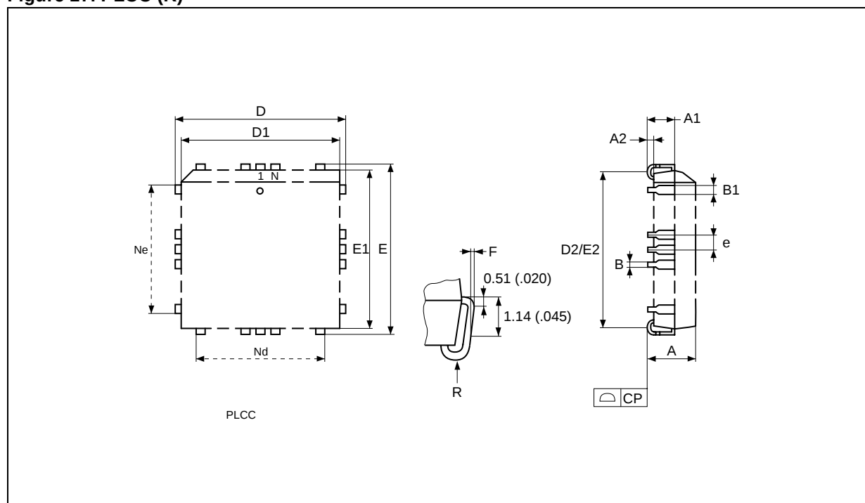
Figure 17. PLCC (K)
