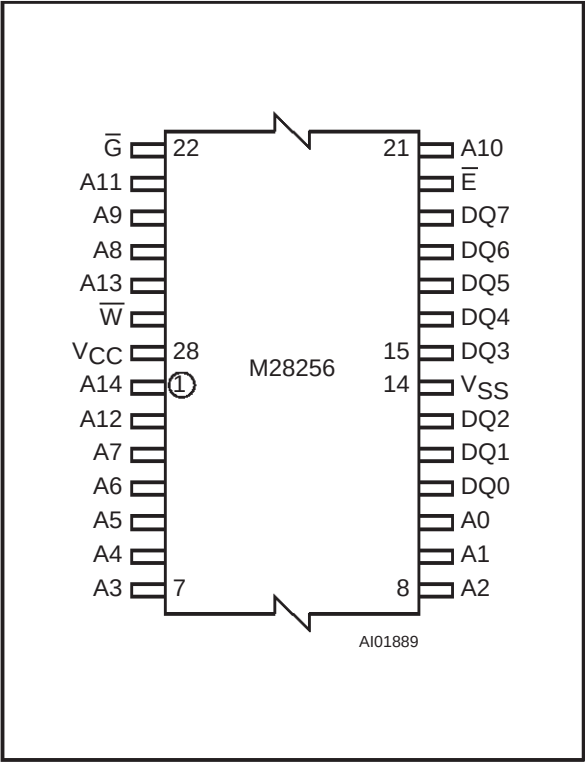
Figure 2D. TSOP Pin Connections
