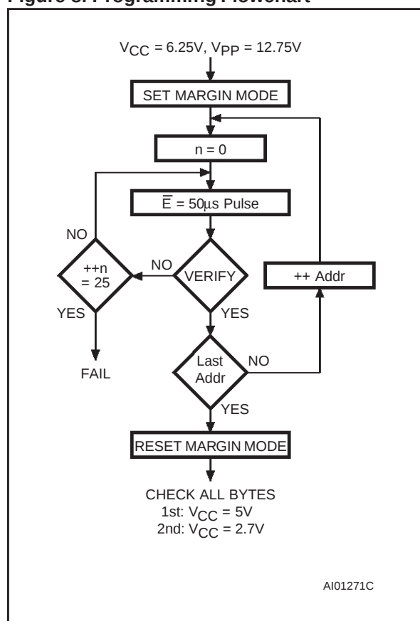
Figure 8. Programming Flowchart
