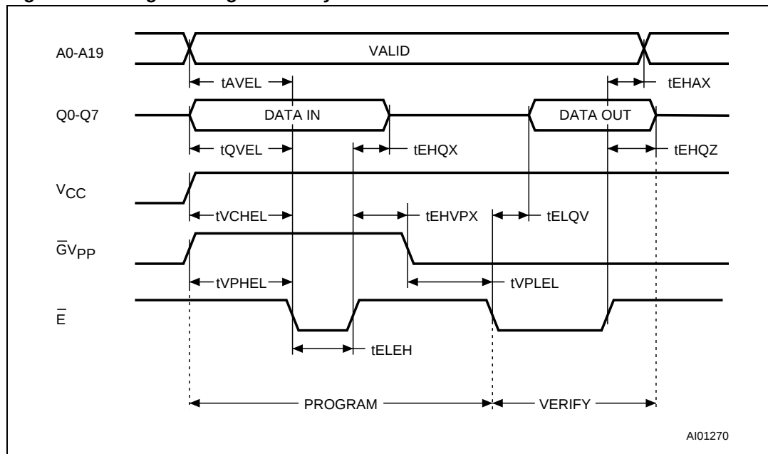
Figure 10. Programming and Verify modes AC waveforms
