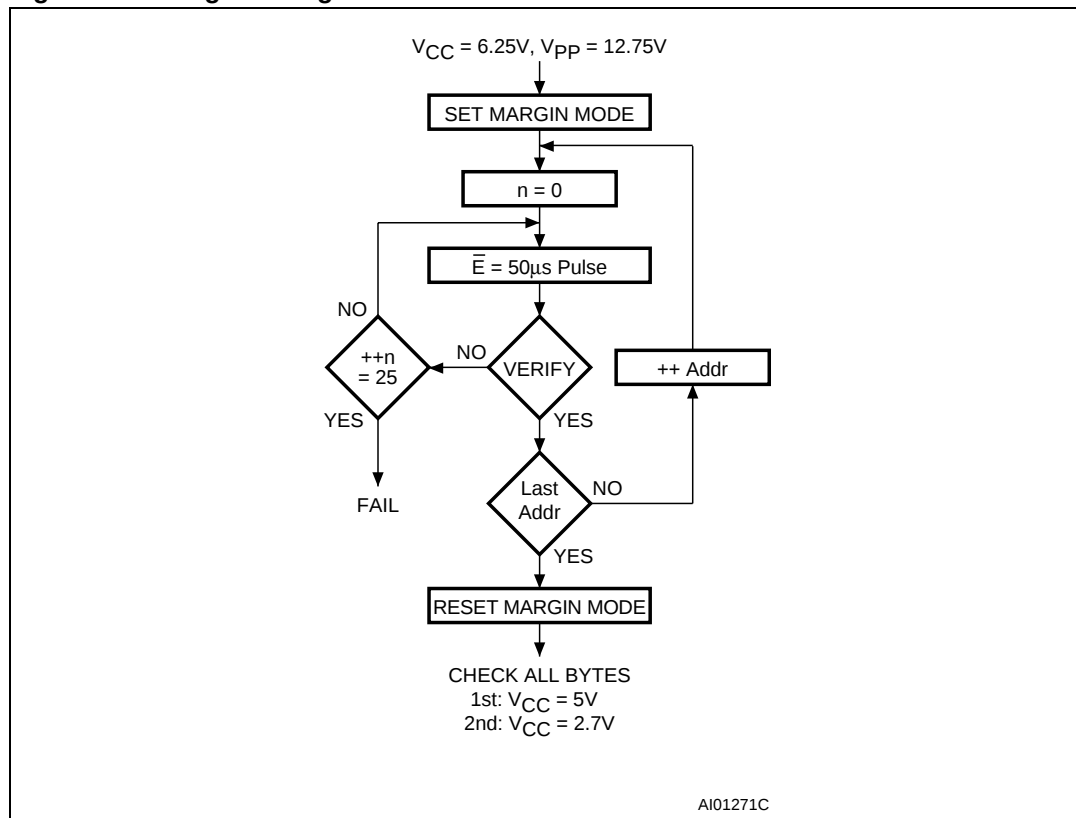
Figure 5. Programming flowchart
