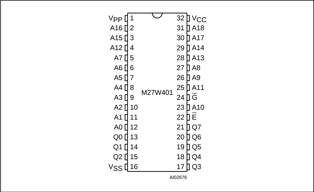
Figure 2. DIP Connections
