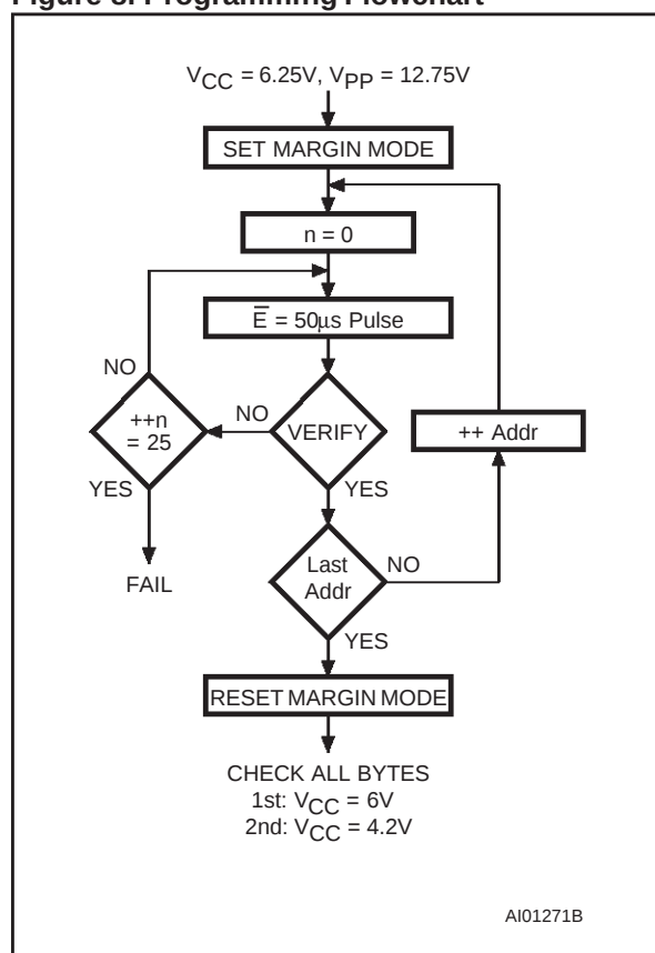
Figure 8. Programming Flowchart
