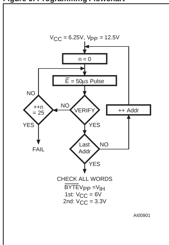
Figure 9. Programming Flowchart
