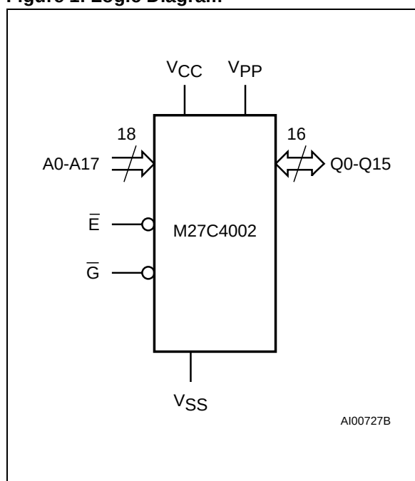
Figure 1. Logic Diagram
