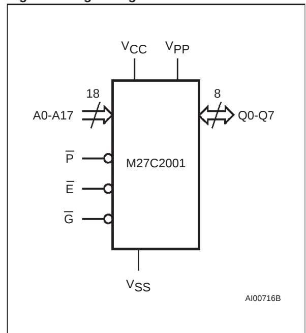
Figure 1. Logic Diagram
